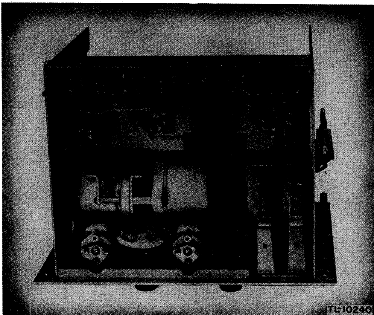
Figure 23. Frequency Meter BC-221-B, bottom view of chassis with coil shield removed.
