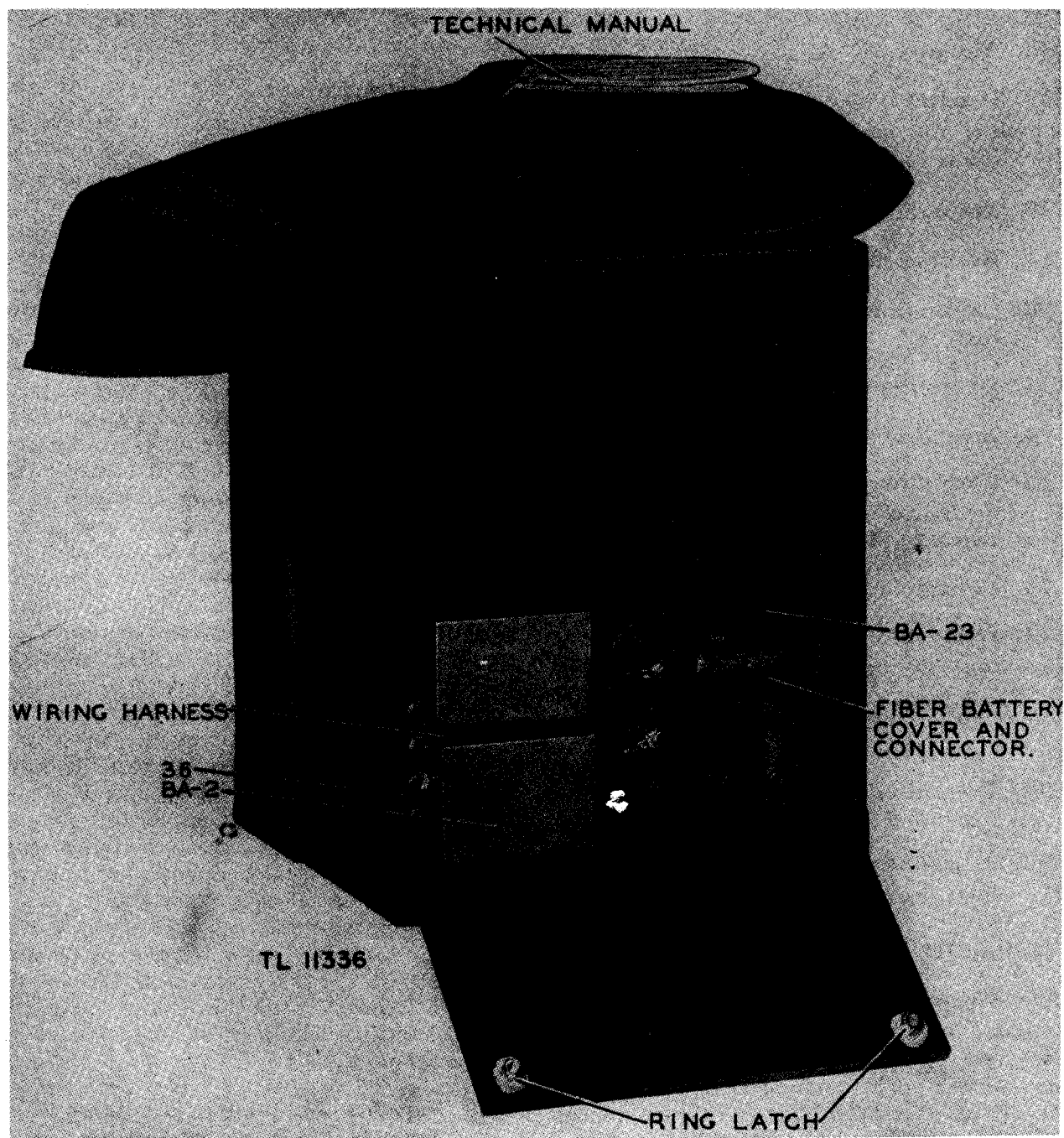
Figure 67. Frequency Meter BC-221-(G), wooden cabinet, battery installation.
