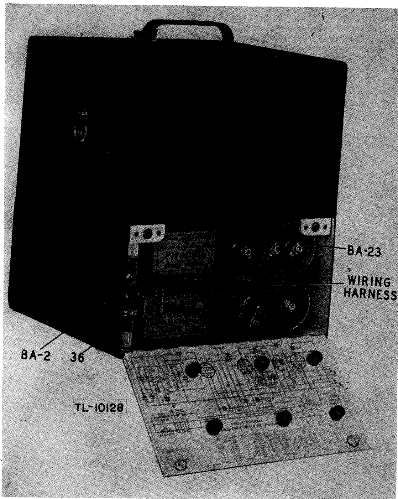
Figure 10. Use of wiring harness with battery installation, in metal cabinet.
