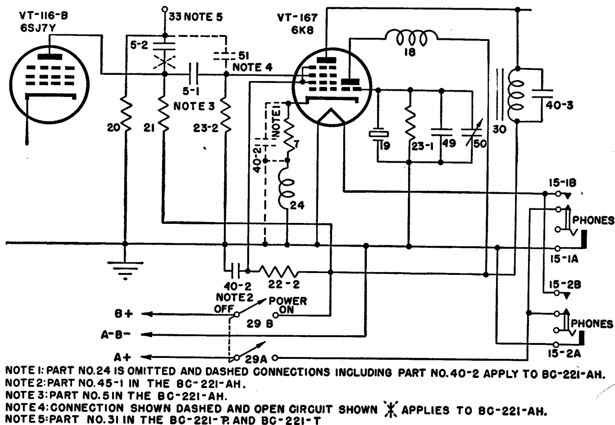
Figure 74. Frequency Meter BC-221-(6), functional diagram, crystal-oscillator circuit.
