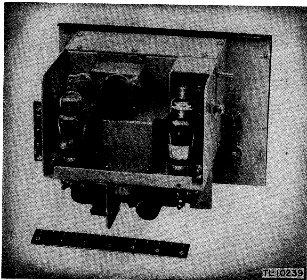
Figure 22. Frequency Meter BC-221-F, rear view of chassis.
