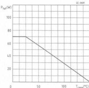
Derating curve
