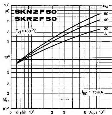
Fig. 5 Recovered charge
