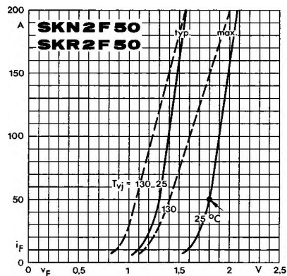
Fig. 8 Forward characteristics
