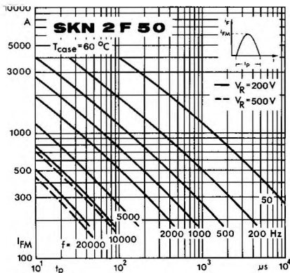
Fig. 1 a Rated sinusoidal peak forward current
