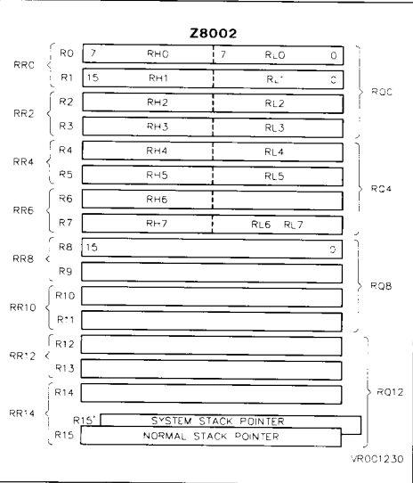
Figure 1-3b. Z8002 General-Purpose Registers
