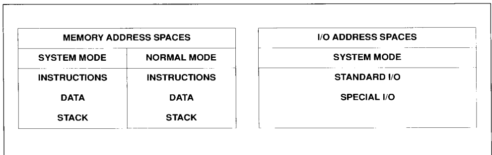
Figure 4-1. Address Spaces on the Z8001 and Z8002
