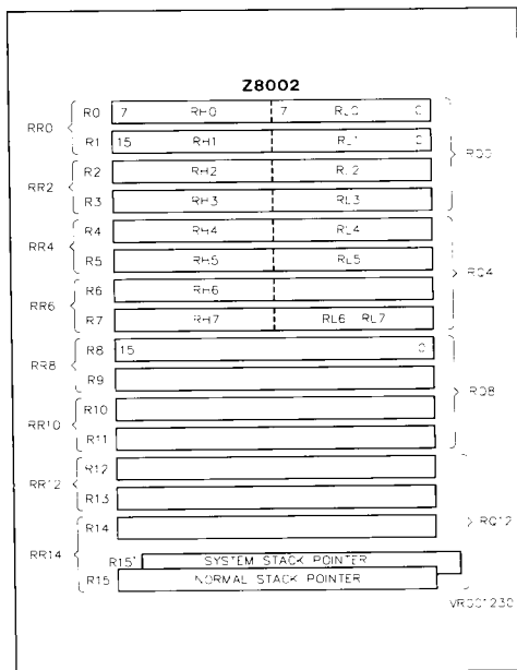
Figure 3-5b. Z8002 General-Purpose Registers (Register Address Space)
