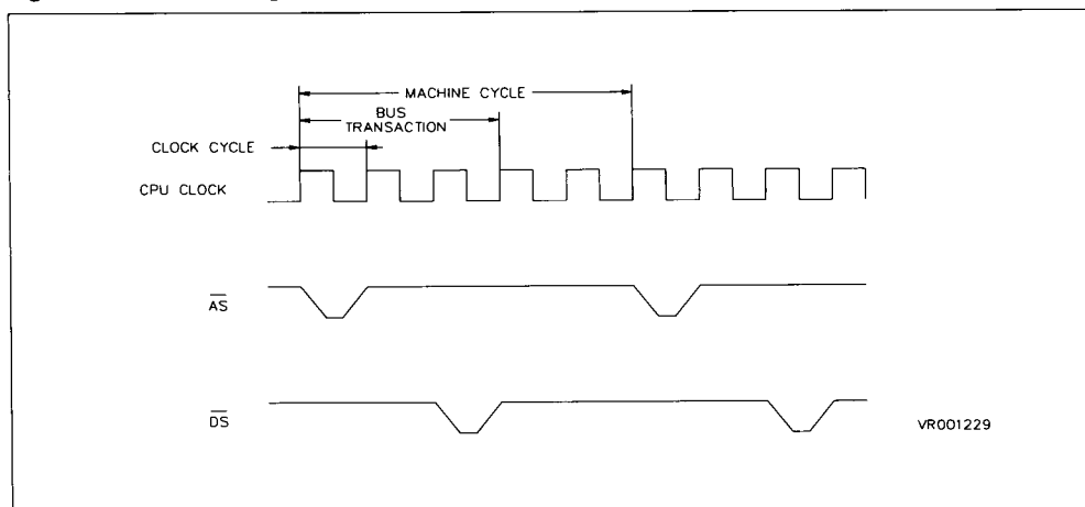
Figure 3-4. Basic Timing Periods
