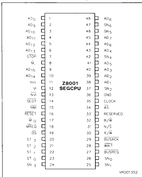
Figure 2-1. Z8001 Pin Configuration
