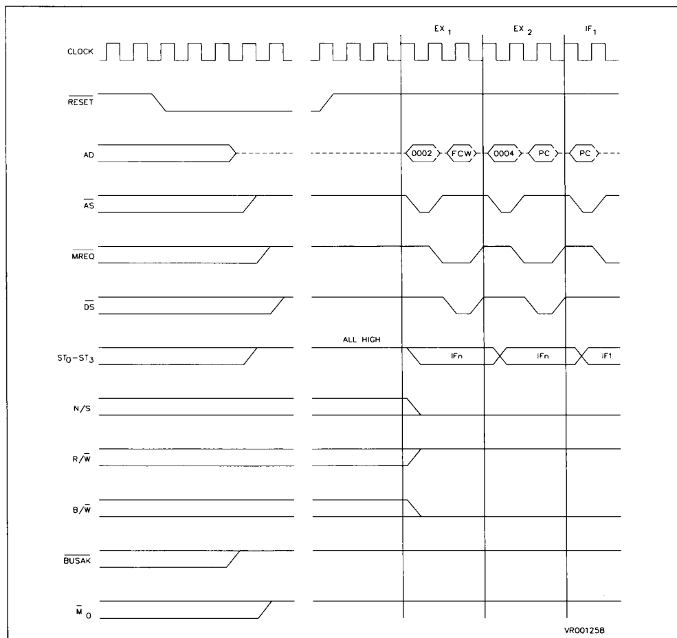
Figure 2-14. Reset Timing
