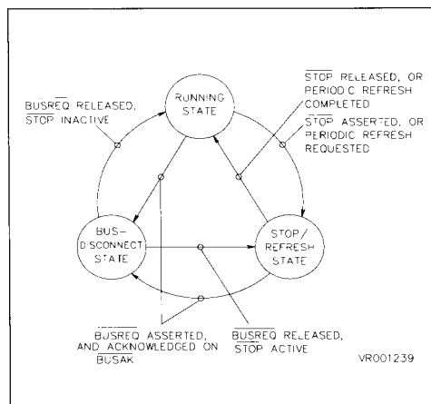
Figure 5-1. Operating States and Transitions
