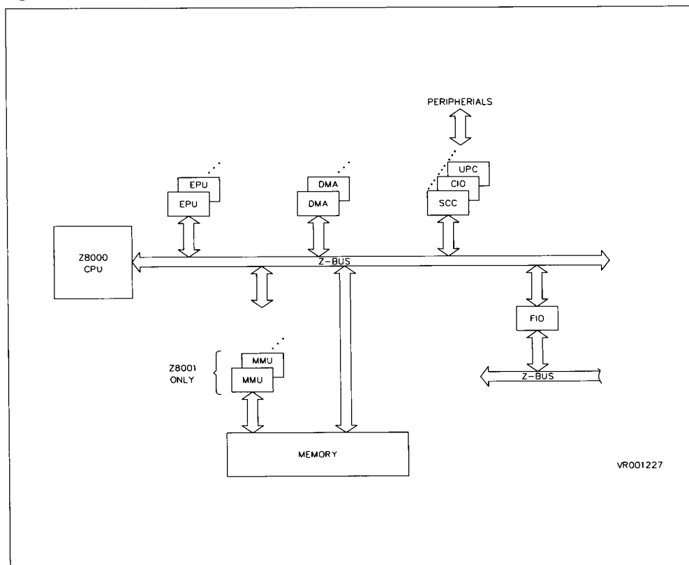
Figure 3-2. Z8000 System Configuration
