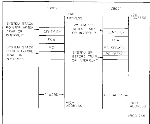
Figure 7-1. Format of Saved Program Status in the System Stack
