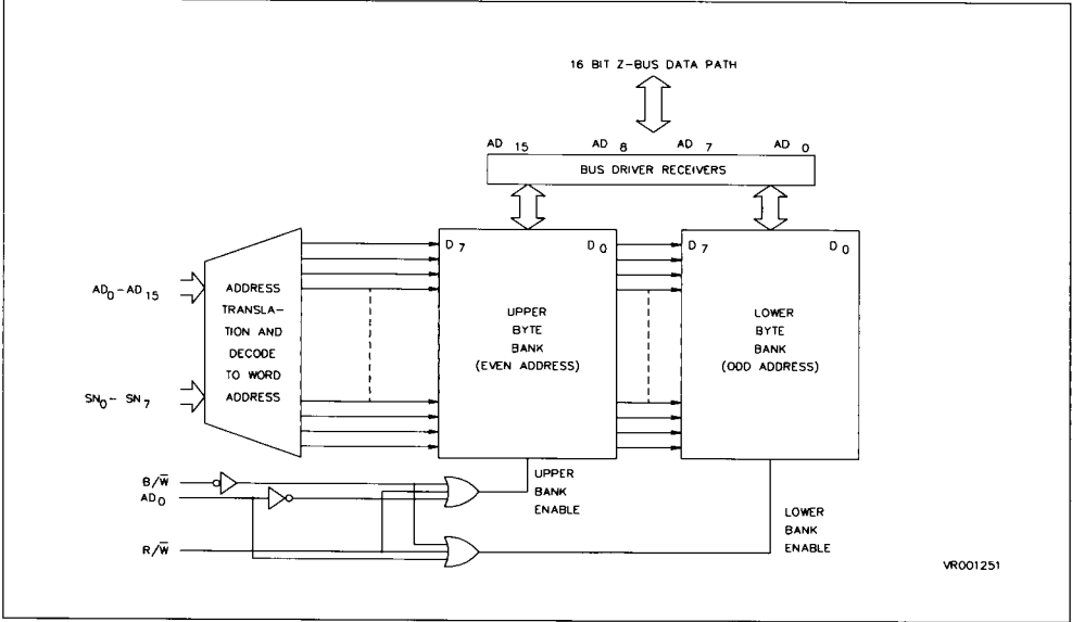
Figure 2-7. Memory Organization
