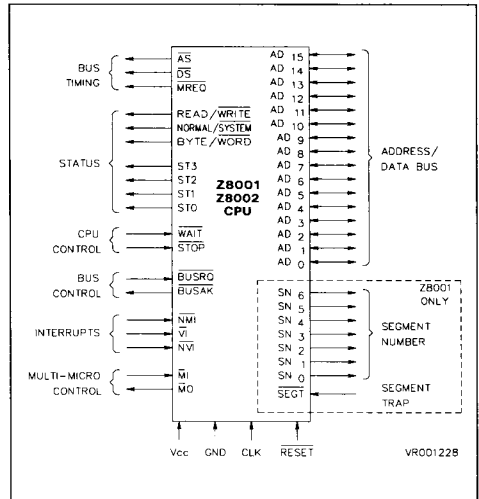
Figure 1-1. Logic Function
