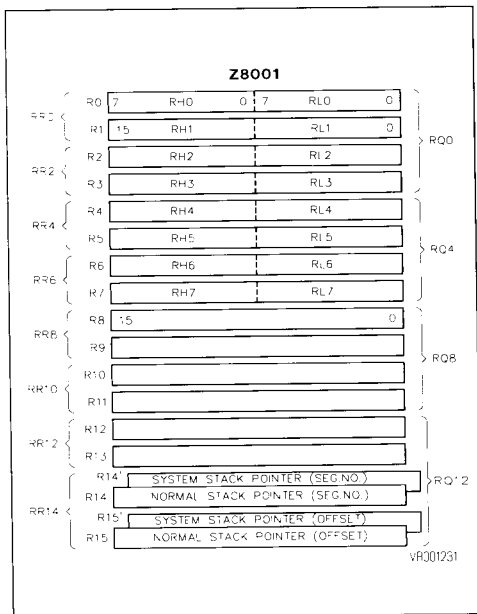
Figure 3-5a. Z8001 General-Purpose Registers (Register Address Space)
