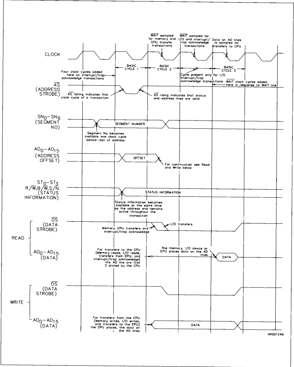
Figure 2-5. Transaction Timing
