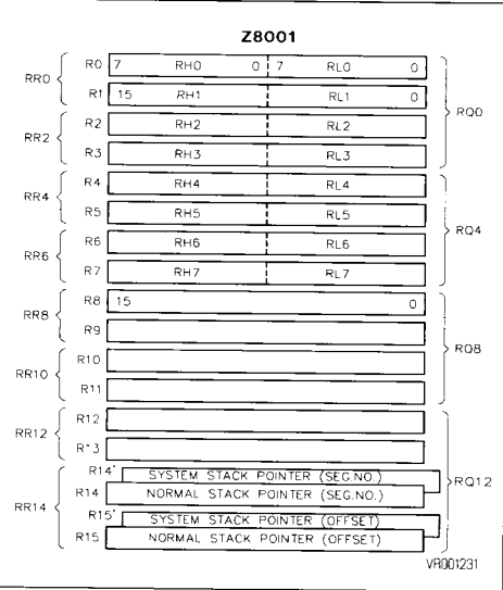
Figure 1-3a. Z8001 General-Purpose Registers
