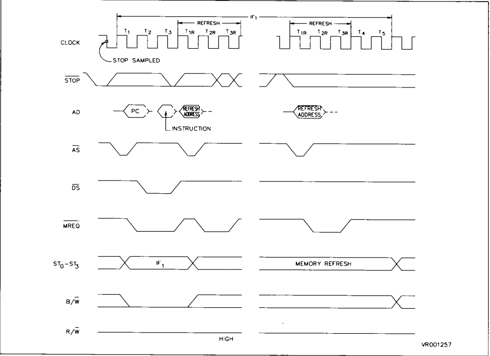
Figure 2-13. Stop Timing
