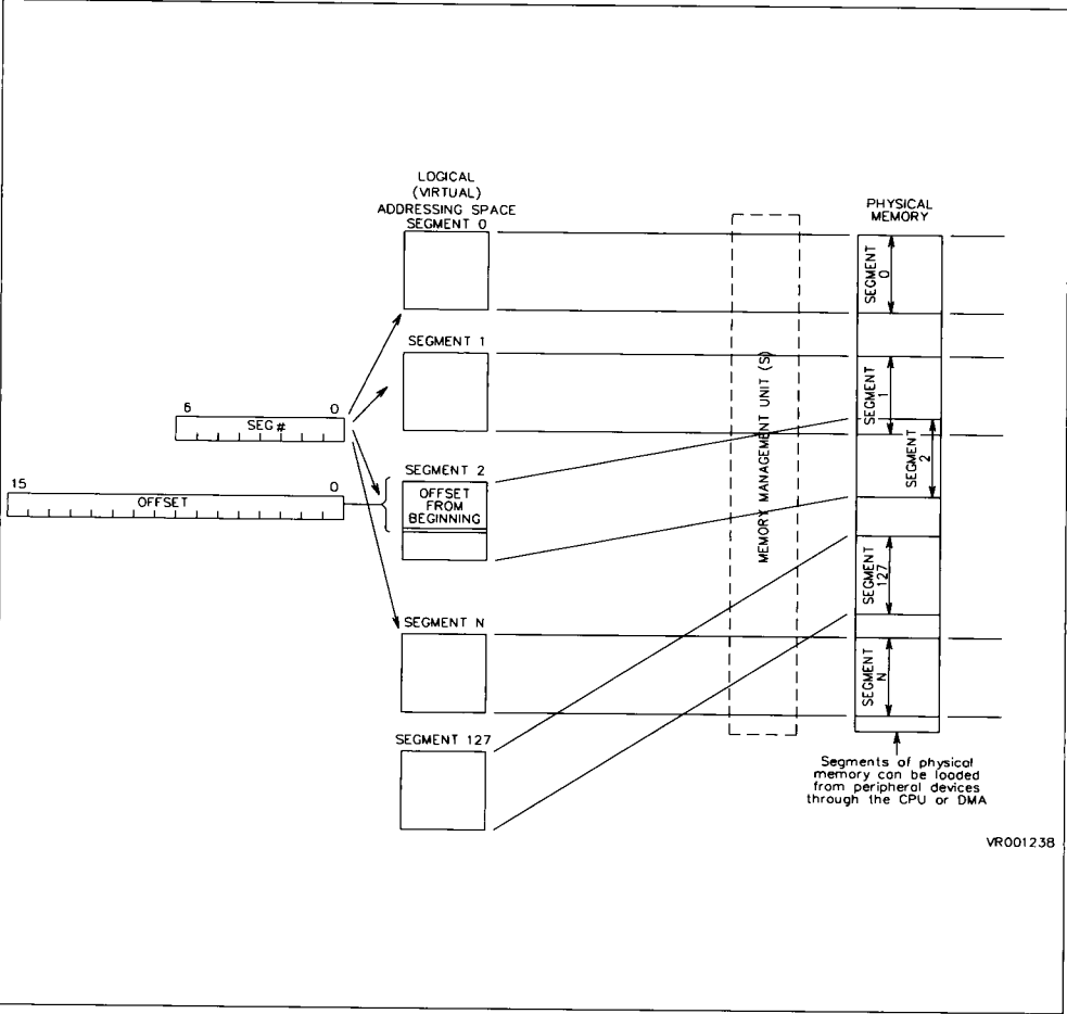
Figure 4-4. Segmented Address Translation
