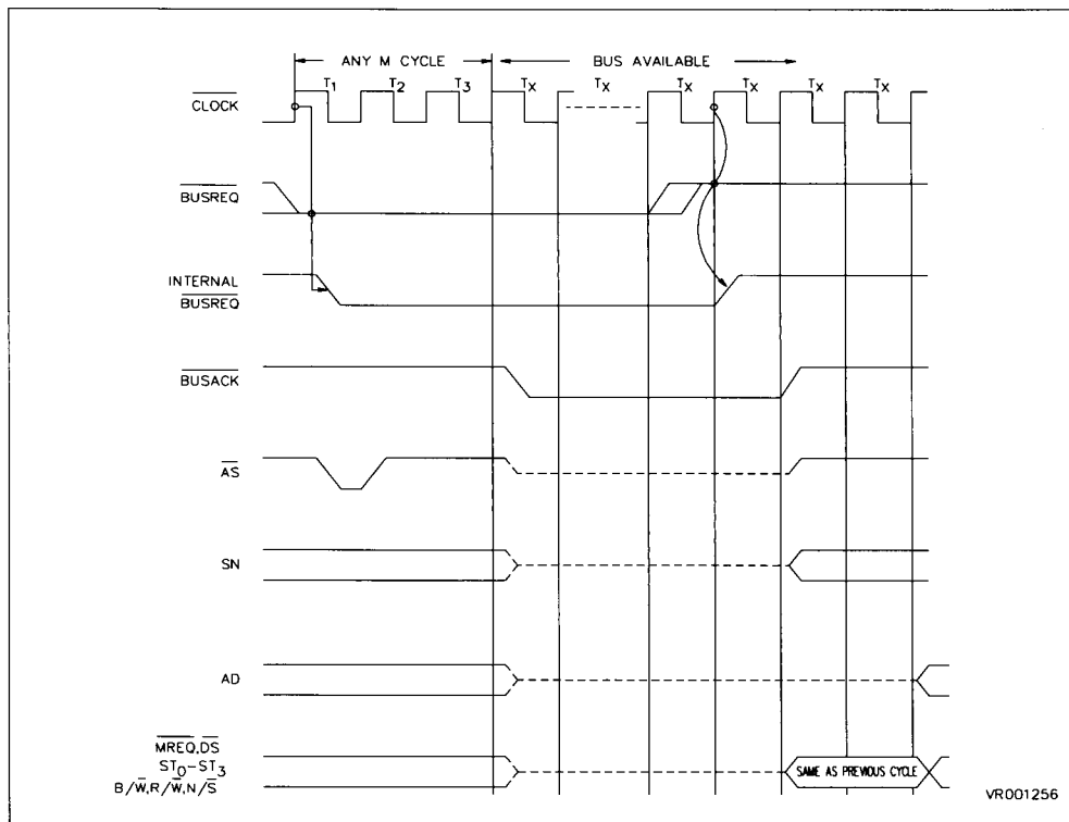
Figure 2-12. Bus Request/Acknowledge Timing
