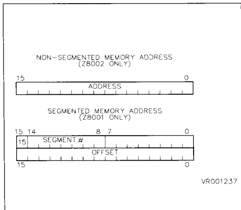
Figure 4-3. Segmented and Nonsegmented Address Formats
