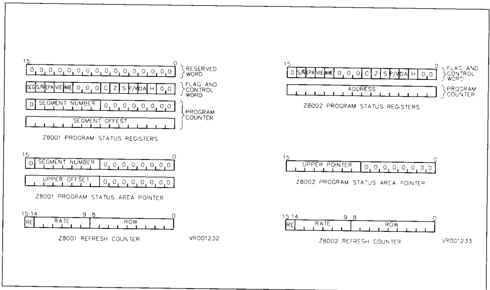
Figure 3-6. CPU Special Registers
