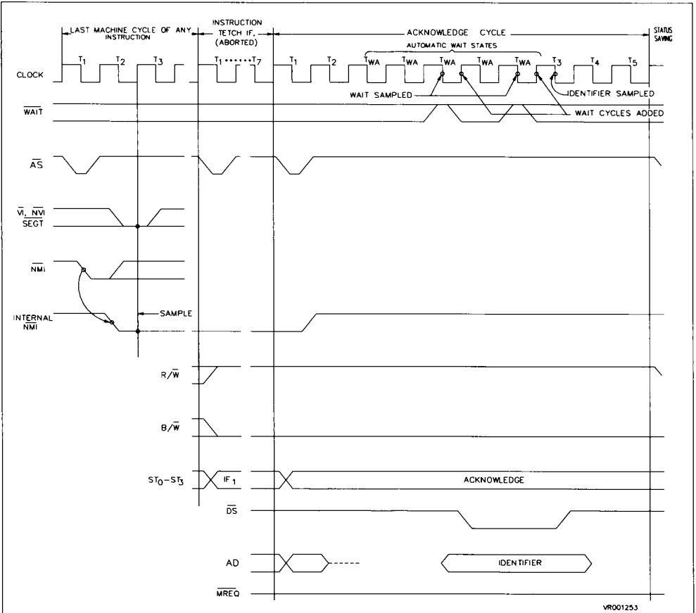
Figure 2-9. Interrupt and Segment Trap Request an Acknowledge Transition
