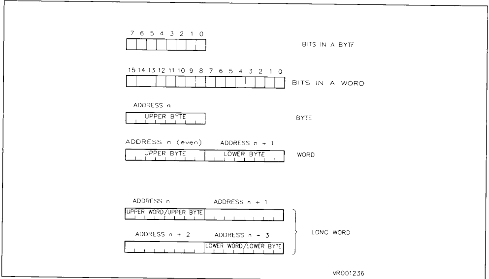
Figure 4-2. Addressable Data Elements
