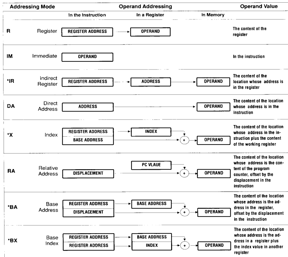
Figure 6-1. Addressing Modes
