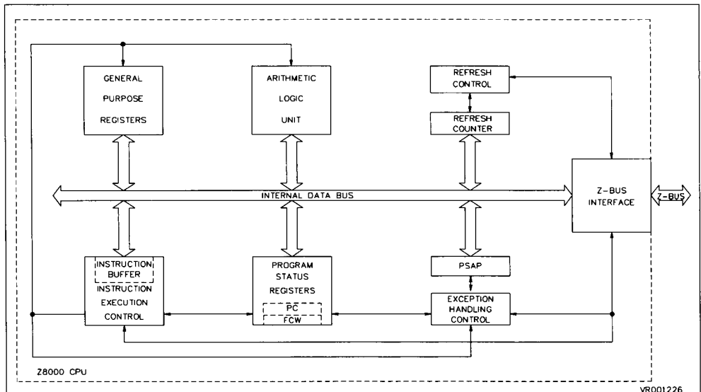
Figure 1-2. Z8000 CPU Functional Block Diagram
