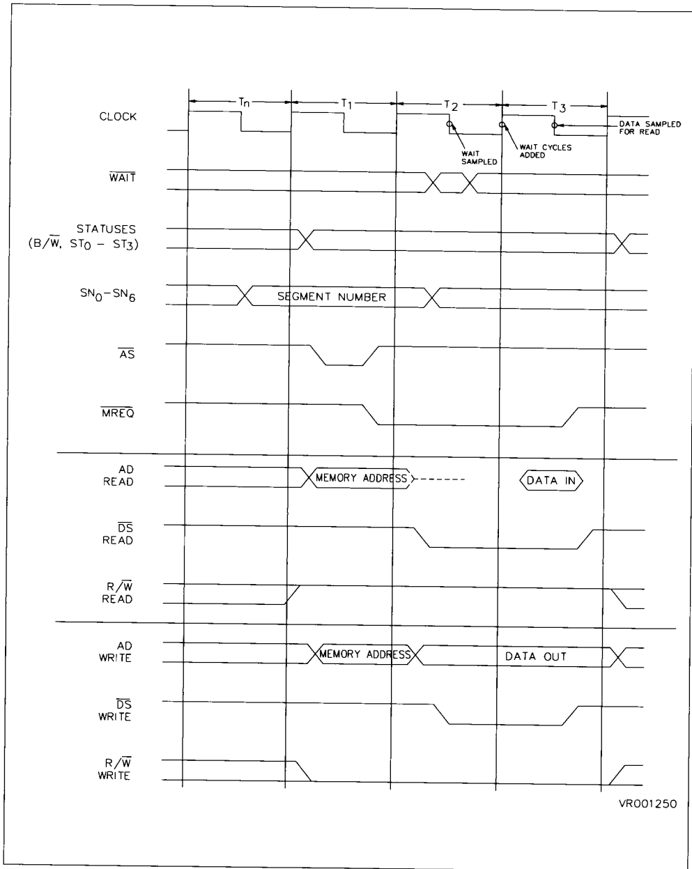
Figure 2-6. Memory Read and Write Transaction
