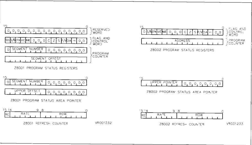
Figure 5-2. Program Status Registers
