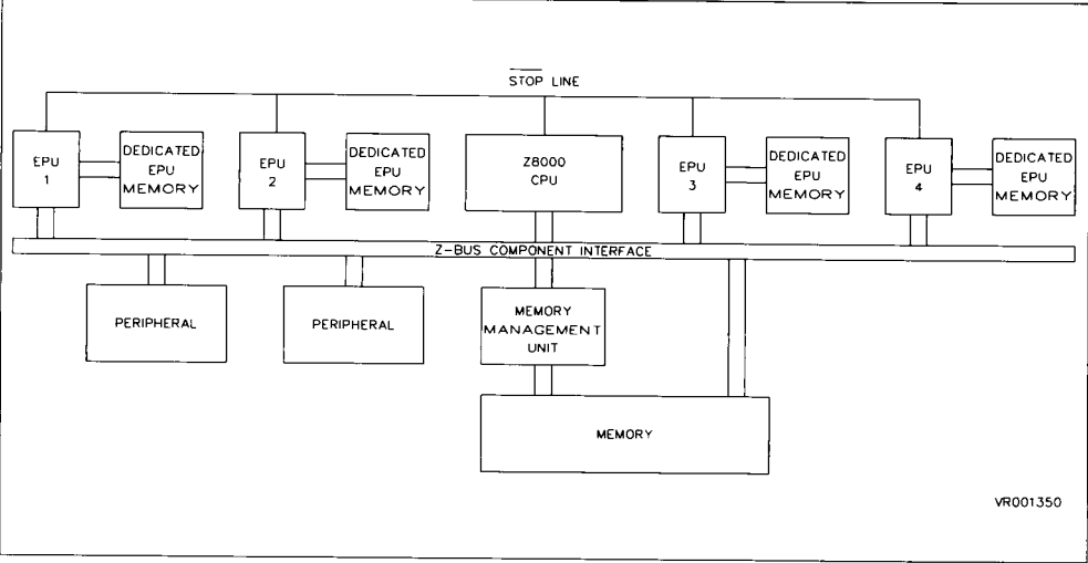
Figure 3-8. Typical Extended Processor Configuration
