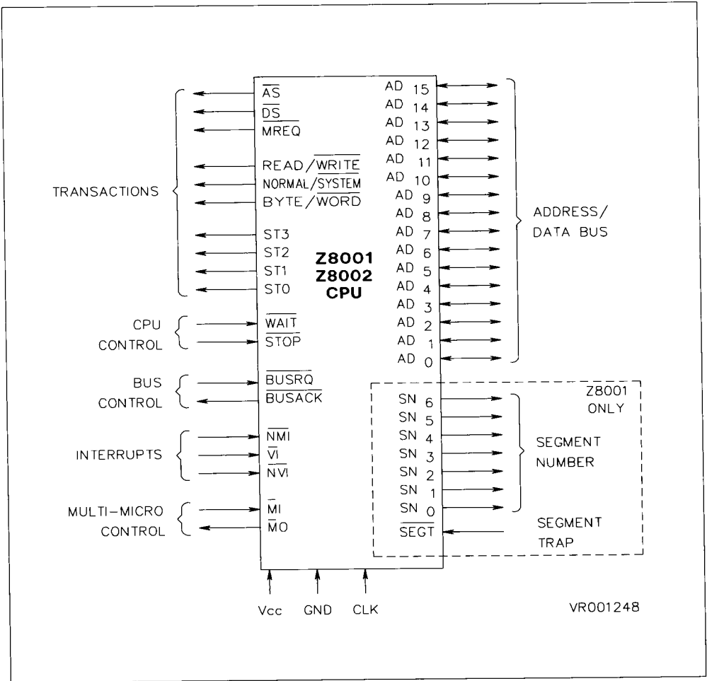
Figure 2-4. Pin Functions
