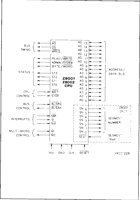
Figure 3-3. Z8000 Pin Functions
