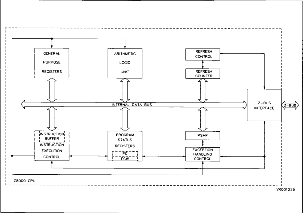
Figure 3-1. Z8000 CPU Functional Block Diagram
