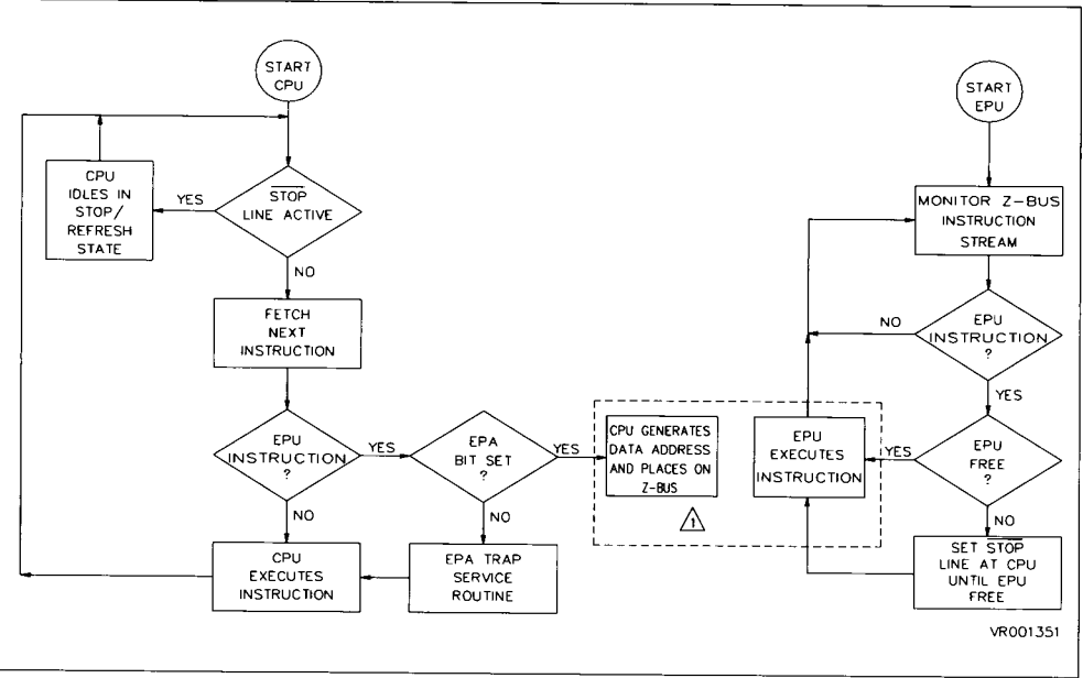
Figure 3-9. EPA and Z8000 CPU Instruction Execution
