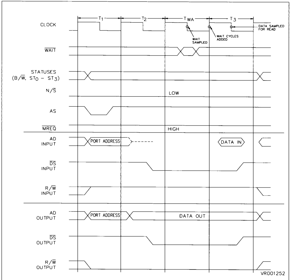
Figure 2-8. Input/Output Transaction
