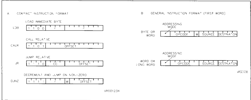
Figure 3-7. Instruction Formats
