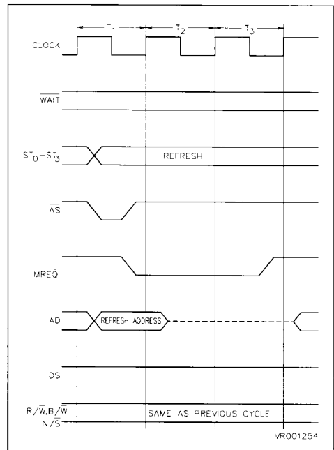
Figure 2-11. Memory Refresh Timing
