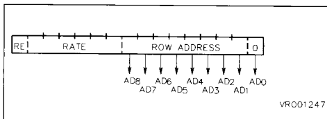
Figure 8-1. Refresh Control Register
