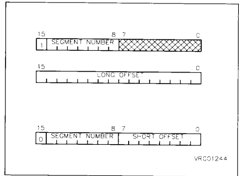
Figure 6-2. Segmented Memory Address Within Instruction
