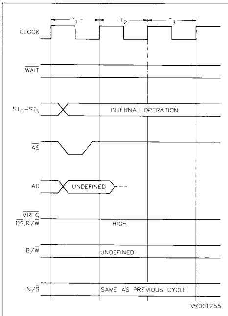
Figure 2-10. Internal Operation Timing
