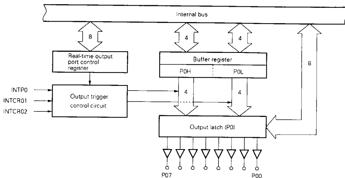
Fig. 3-2 Configuration of Real-Time Output Port
