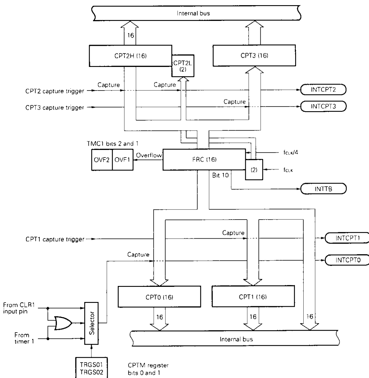
Fig. 3-6 Configuration of the Free Running Counter
