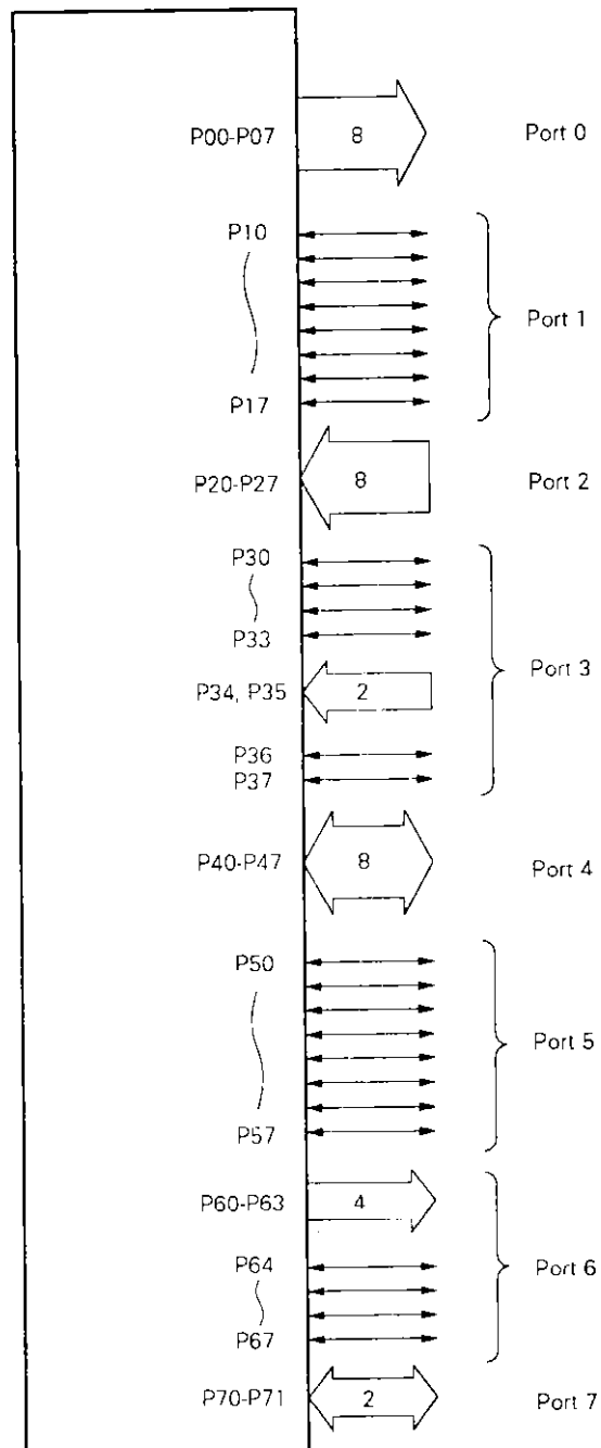
Fig. 3-1 Port Configuration
