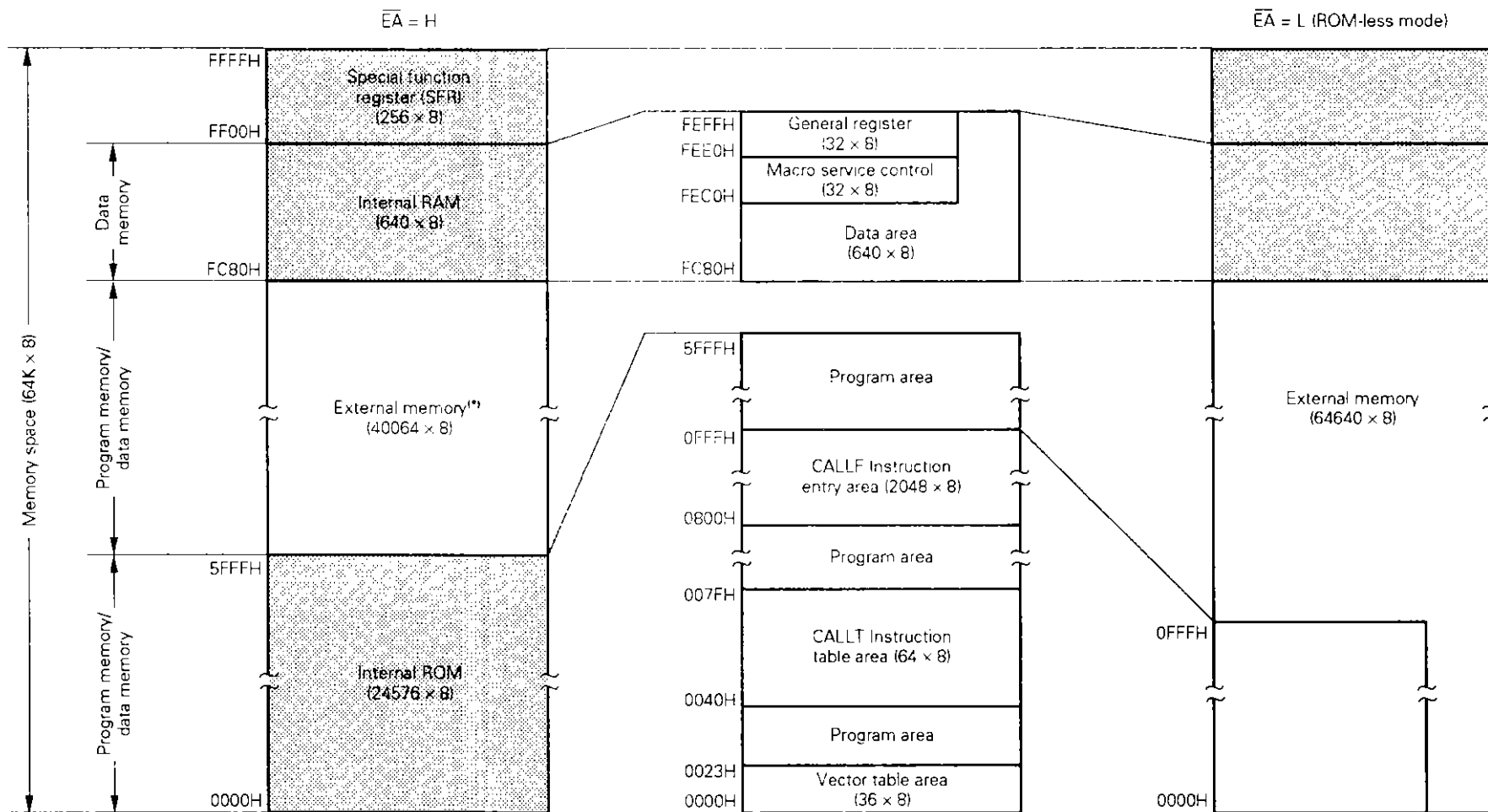
Fig. 2-2 Memory Map ( \mu PD78136)
