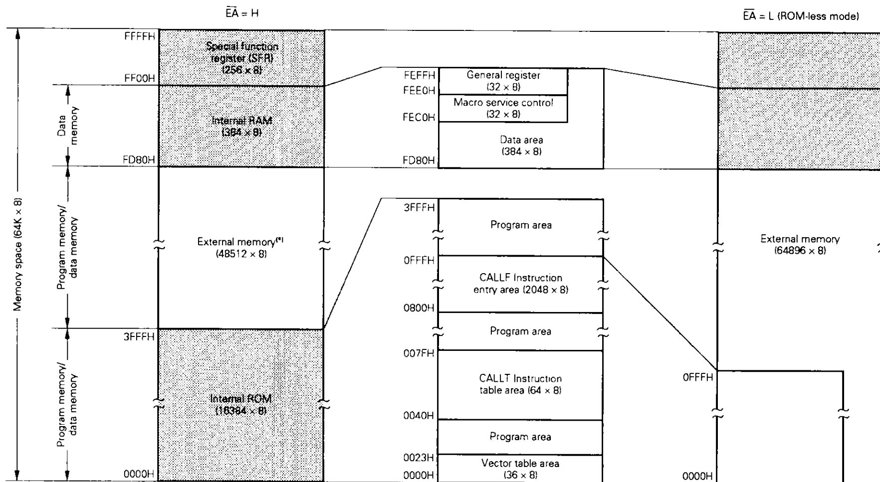
Fig. 2-1 Memory Map (μPD78134A)
