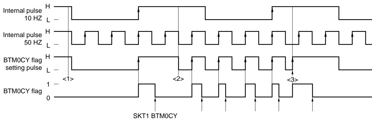
Figure 13-6. Changing BTM0CY Flag Setting Pulse
