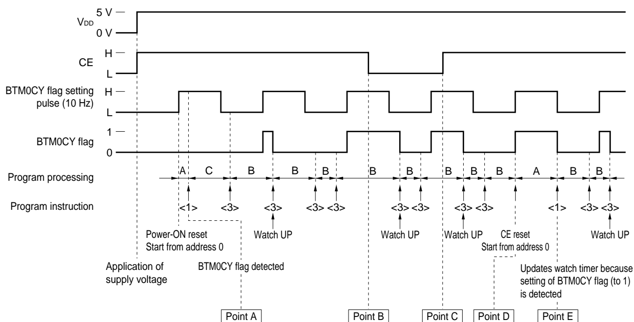
Figure 13-9. Timing Chart
