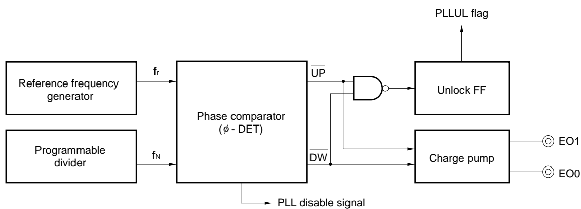
Figure 17-7. Configuration of Phase Comparator, Charge Pump, and Unlock FF
