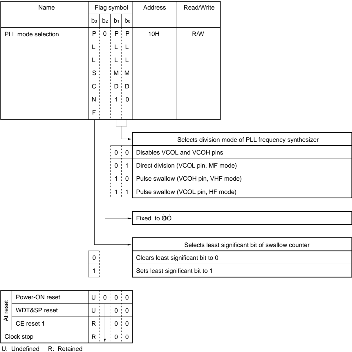
Figure 17-3. Configuration of PLL Mode Selection Register
