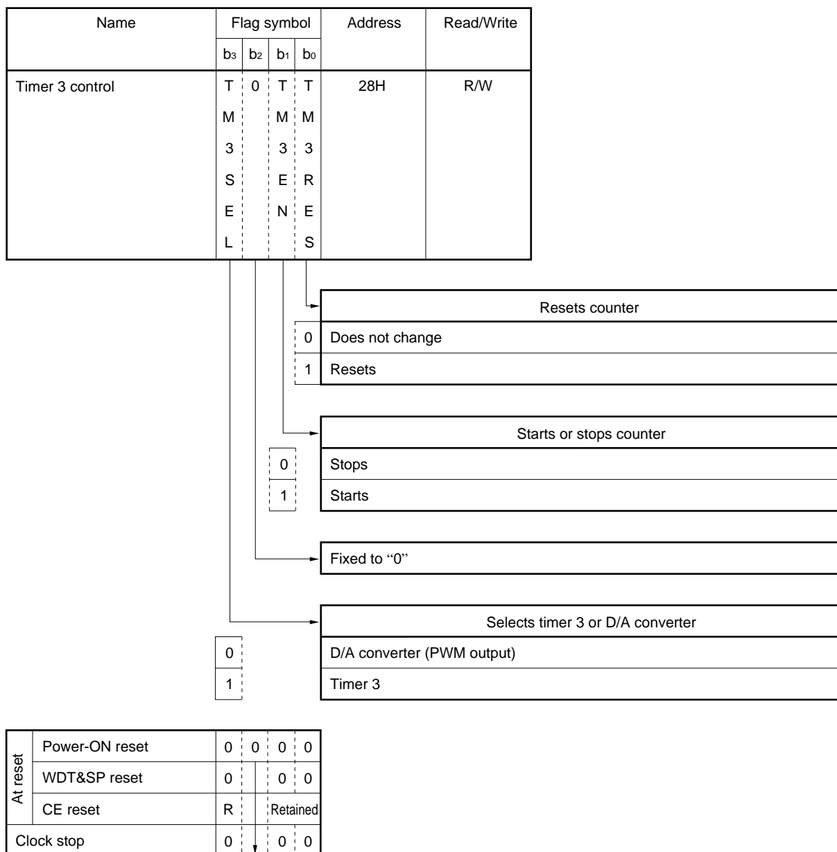
Figure 15-5. Configuration of Timer 3 Control Register
