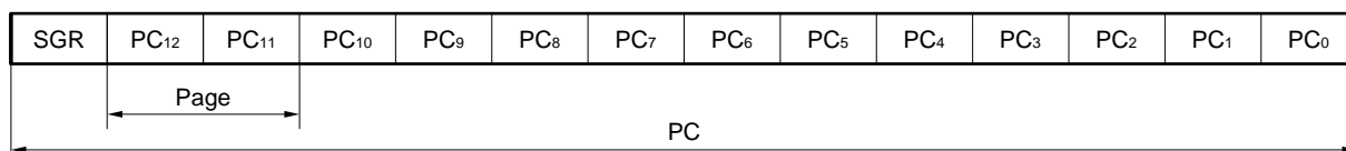
Figure 2-3. Configuration of Program Counter
