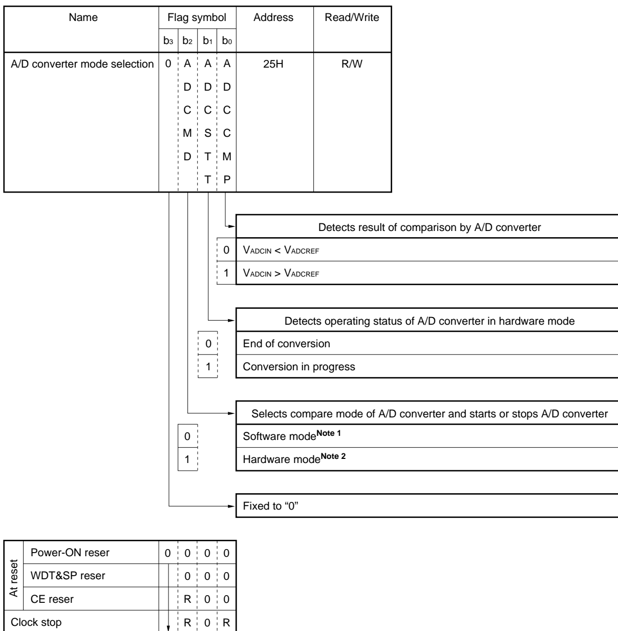
Figure 14-5. Configuration of A/D Converter Mode Selection Register
