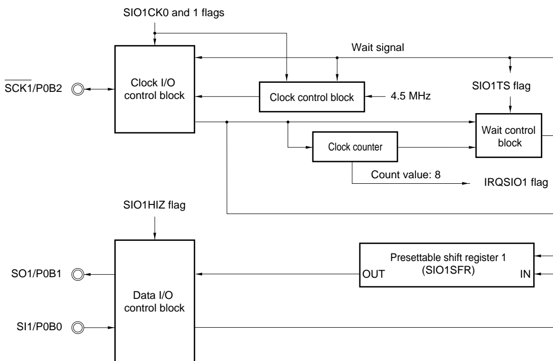
Figure 16-16. Outline of Serial Interface 1
