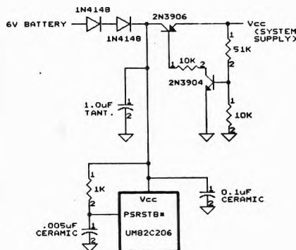
Figure 10. Power Conversion and Reset Circuitry
