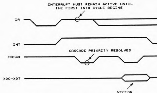
Figure 7. Interrupt Sequence
