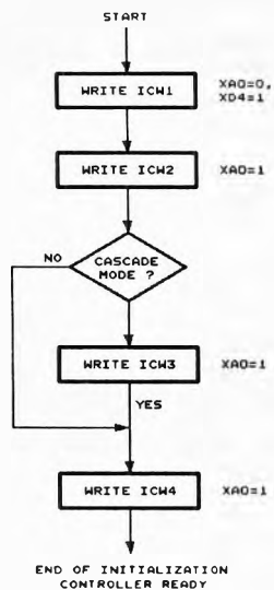
Figure 8. Initialization Sequence
