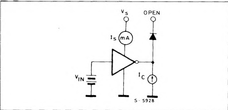
Figure 10 : Input Current as a Function of Input Voltage.
