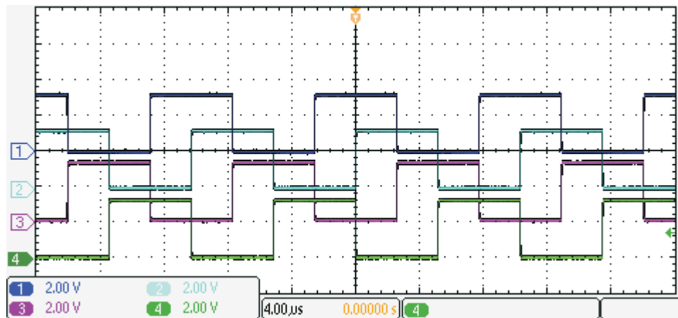
Figure 18. Multiphase PWMs
