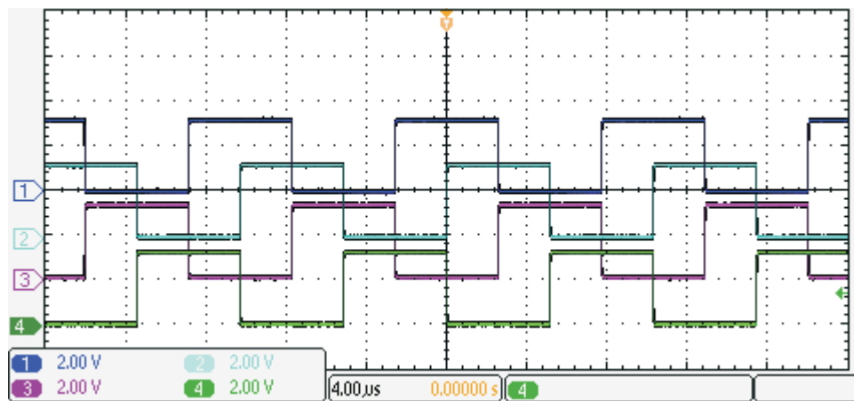
Figure 20. Multiphase PWMs
