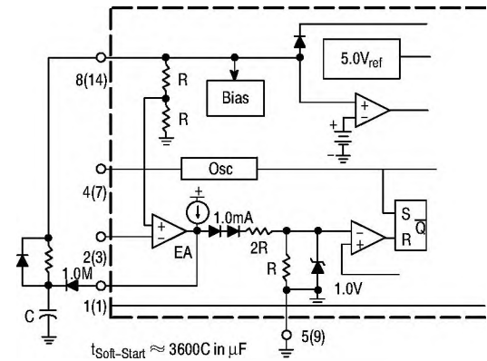
Figure 24. Soft-Start Circuit
