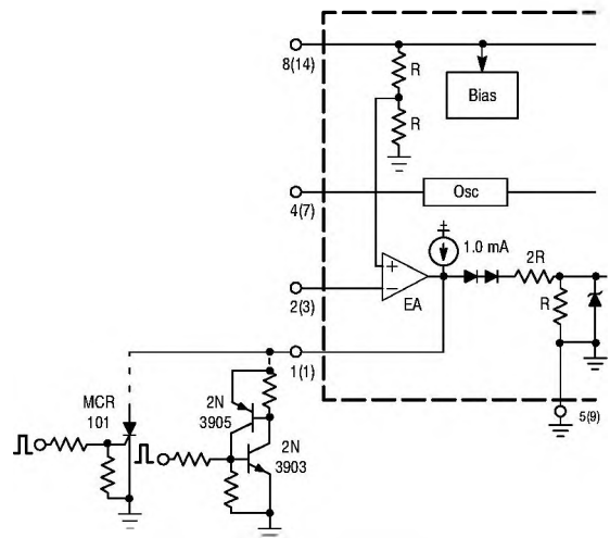
The MCR101 SCR must be selected for a holding of < 0.5 \text{ mA} @ T_A(\text{min}) . The simple two transistor circuit can be used in place of the SCR as shown. All resistors are 10 \text{ k} .
