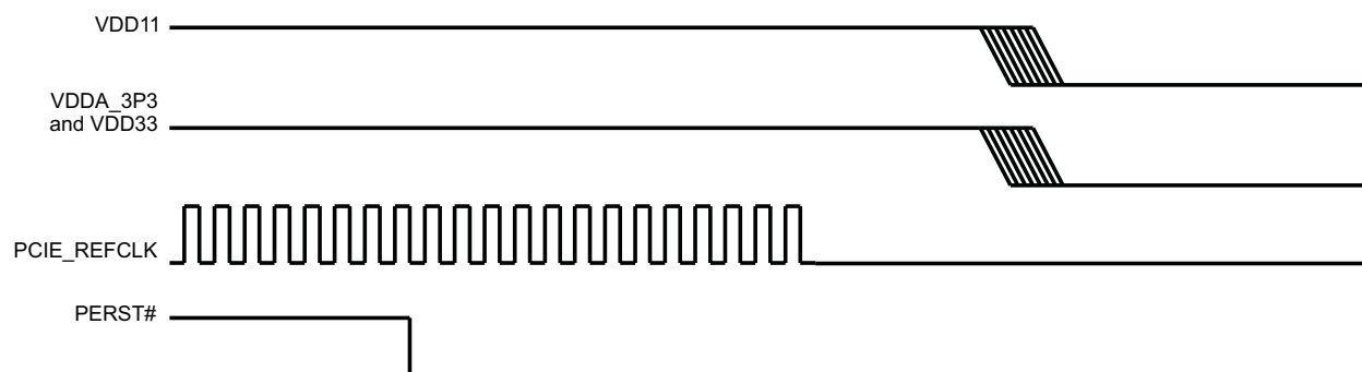
Figure 3-2. Power-Down Sequence
