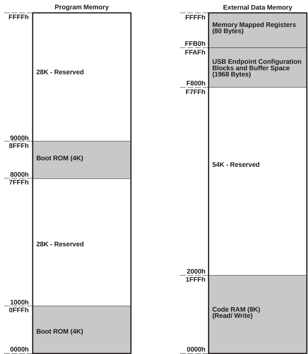
Figure A-1. Boot Loader Mode Memory Map
