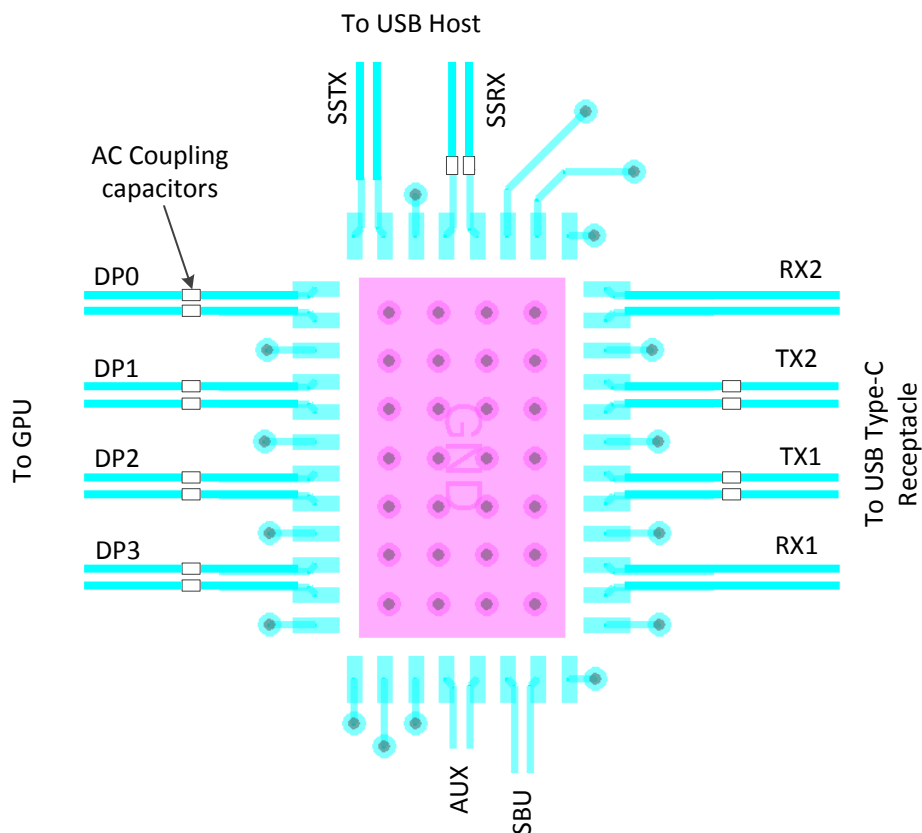
Figure 35. Layout Example
