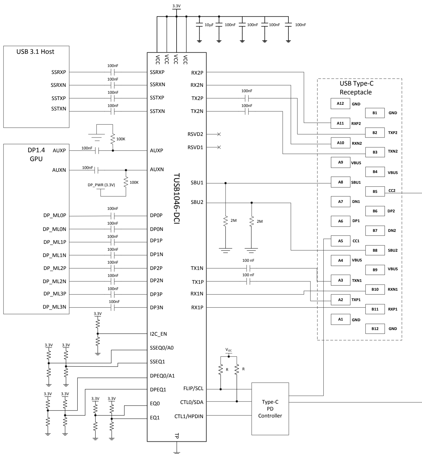
Figure 27. Application Circuit
