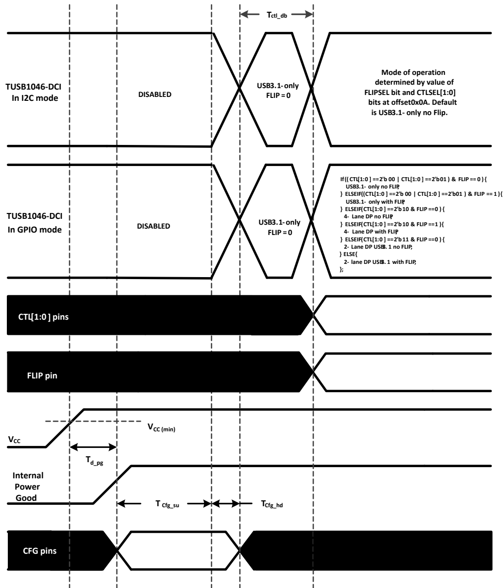
Figure 17. Power-Up Timing
