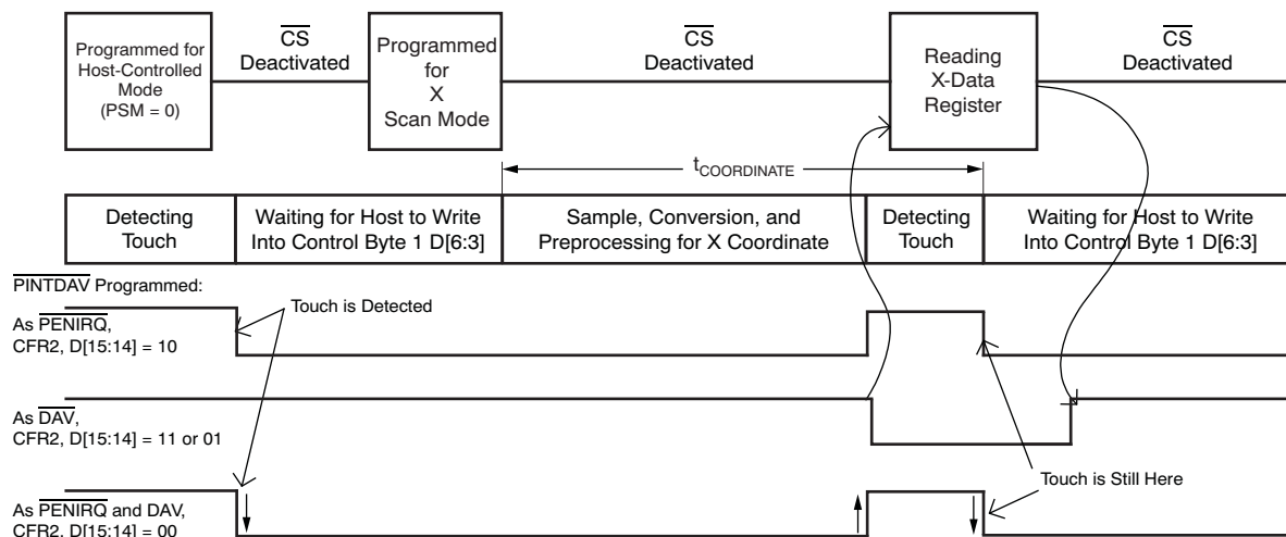
Figure 38. Example of a Single X Coordinate Touch Screen Scan (with Panel Stabilization Time) using TSMODE 3
