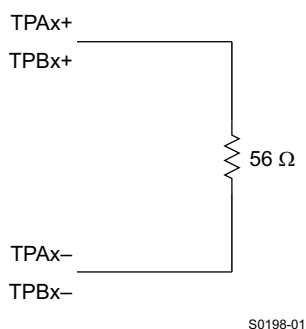
Figure 2-1. Test Load Diagram
