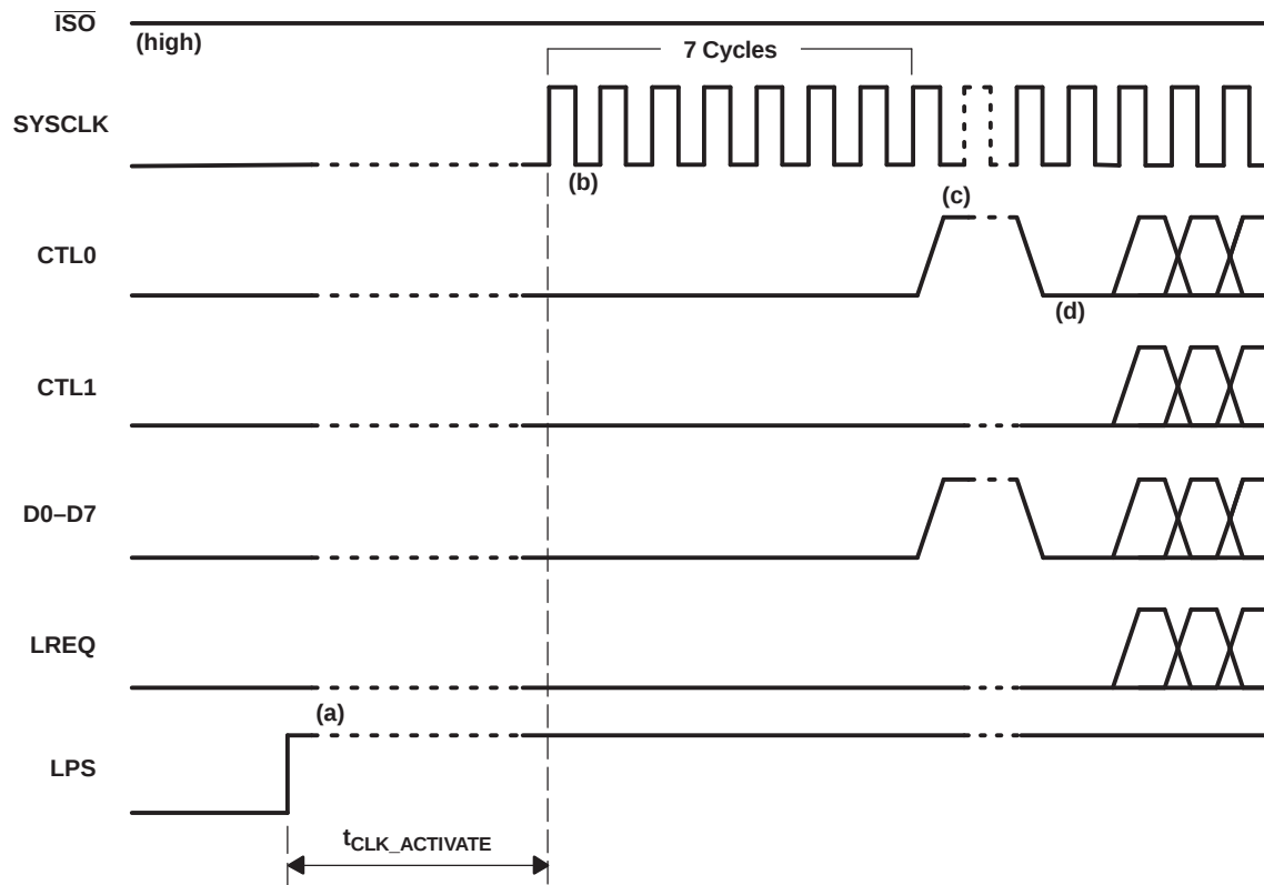
Figure 19. Interface Initialization
