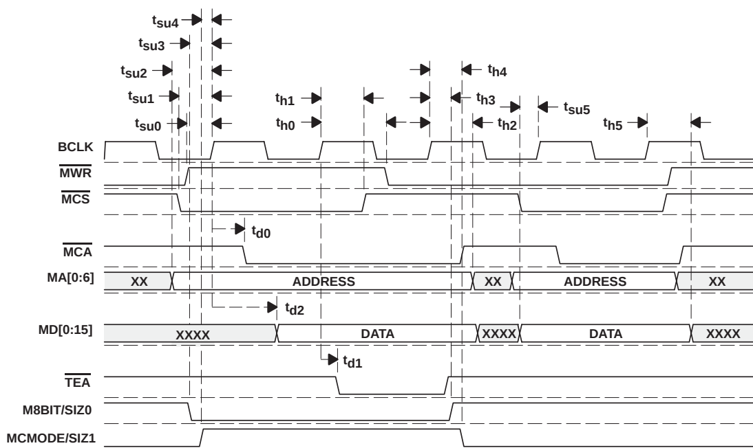
Figure 3-15. Microcontroller Timing
