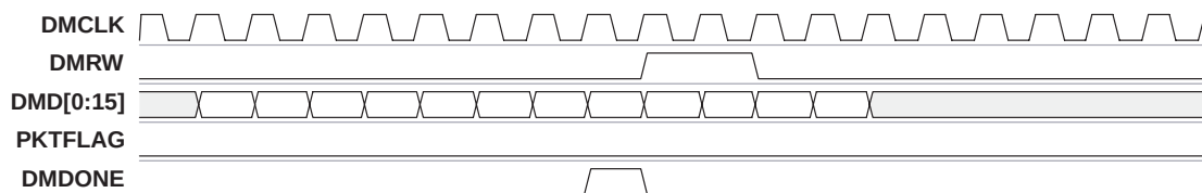
Figure 5–27. Asynchronous Quadlet Receive With Automatic Header and Trailer Removal at 400 Mbps
