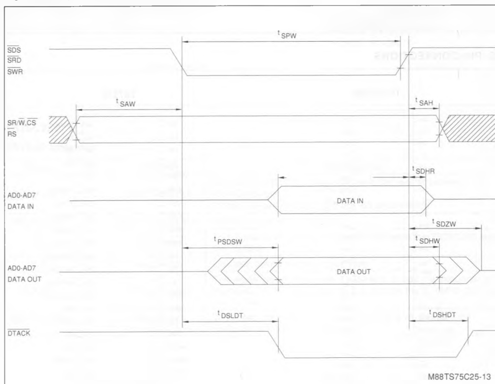
Figure 12 : System Bus Timing Diagram.
