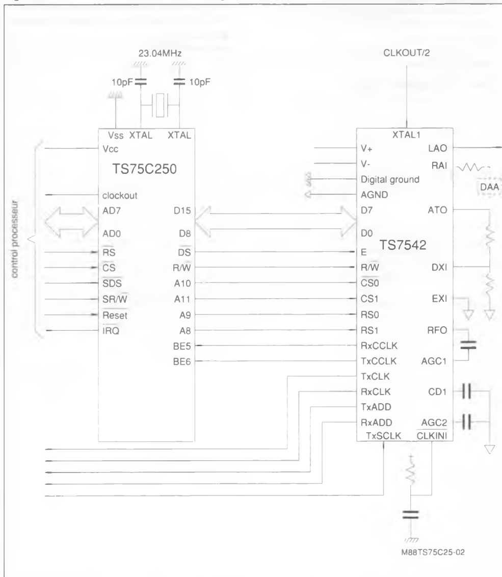
Figure 2 : Interconnections between the Analog Front End Chip and the Digital Signal Processor TS75C250.
