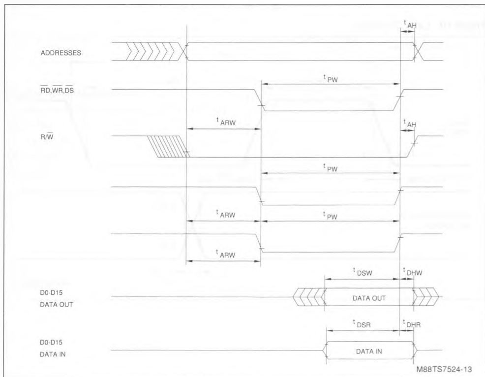
Figure 11 : Local Bus Timing Diagram.
