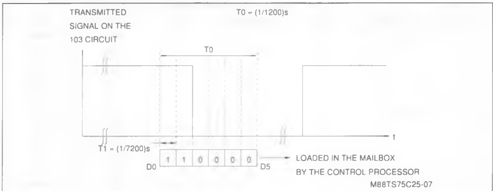
Figure 7 : FSK Mode.
