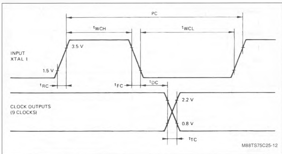
Figure 10 : Clock Generator.
