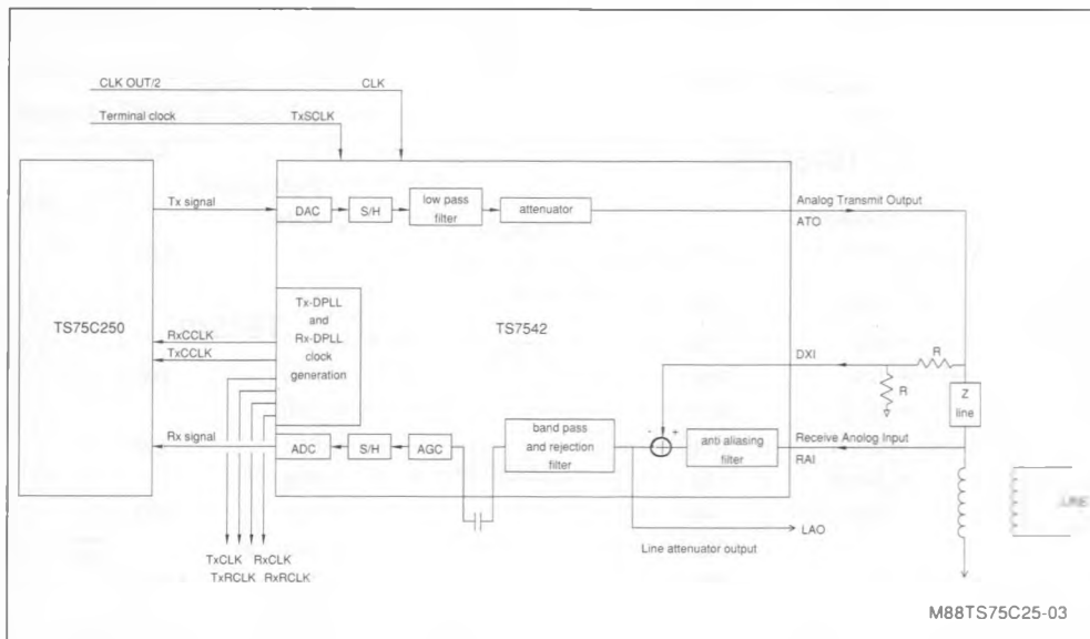
Figure 3 : TS7542 Block Diagram.
