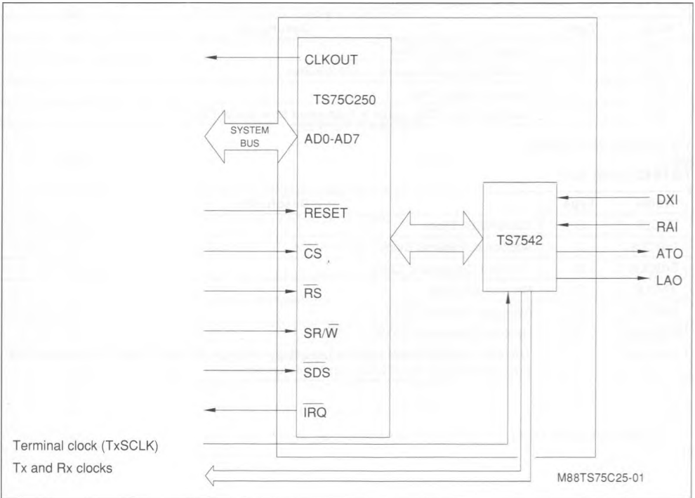
Figure 1 : TS75C25 Block Diagram.
