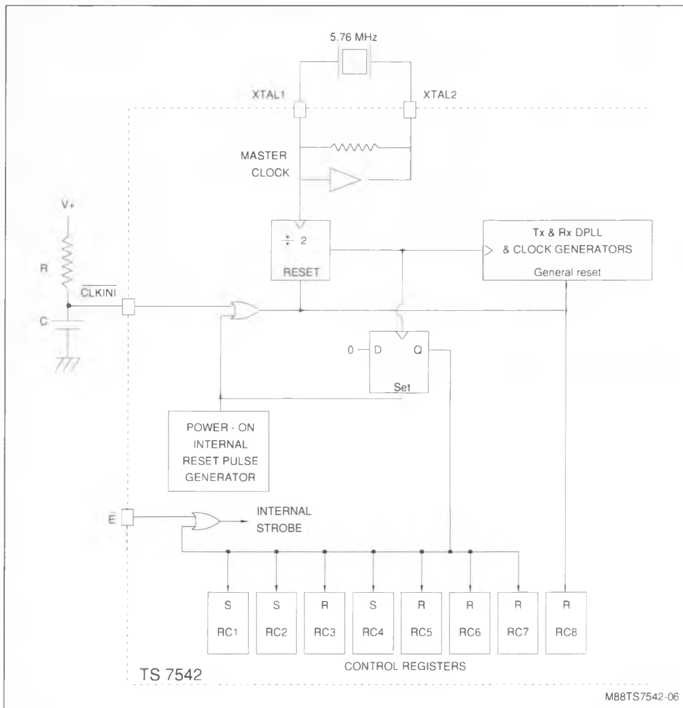
Figure 4 : Power-on Initialization Circuitry.
