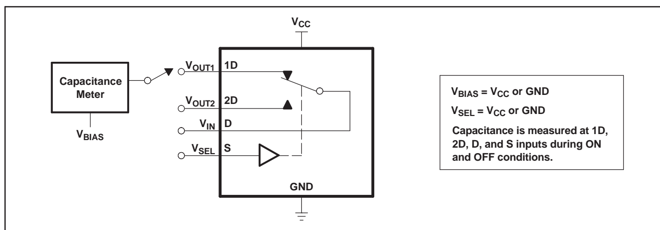
Figure 15. Capacitance
