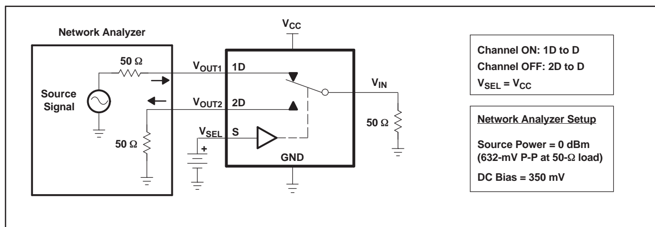
Figure 9. Crosstalk ( X_{TALK} )
