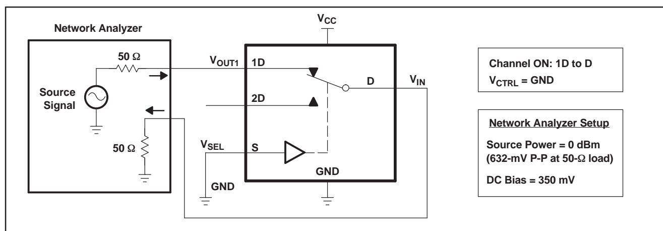
Figure 10. Bandwidth (BW)
