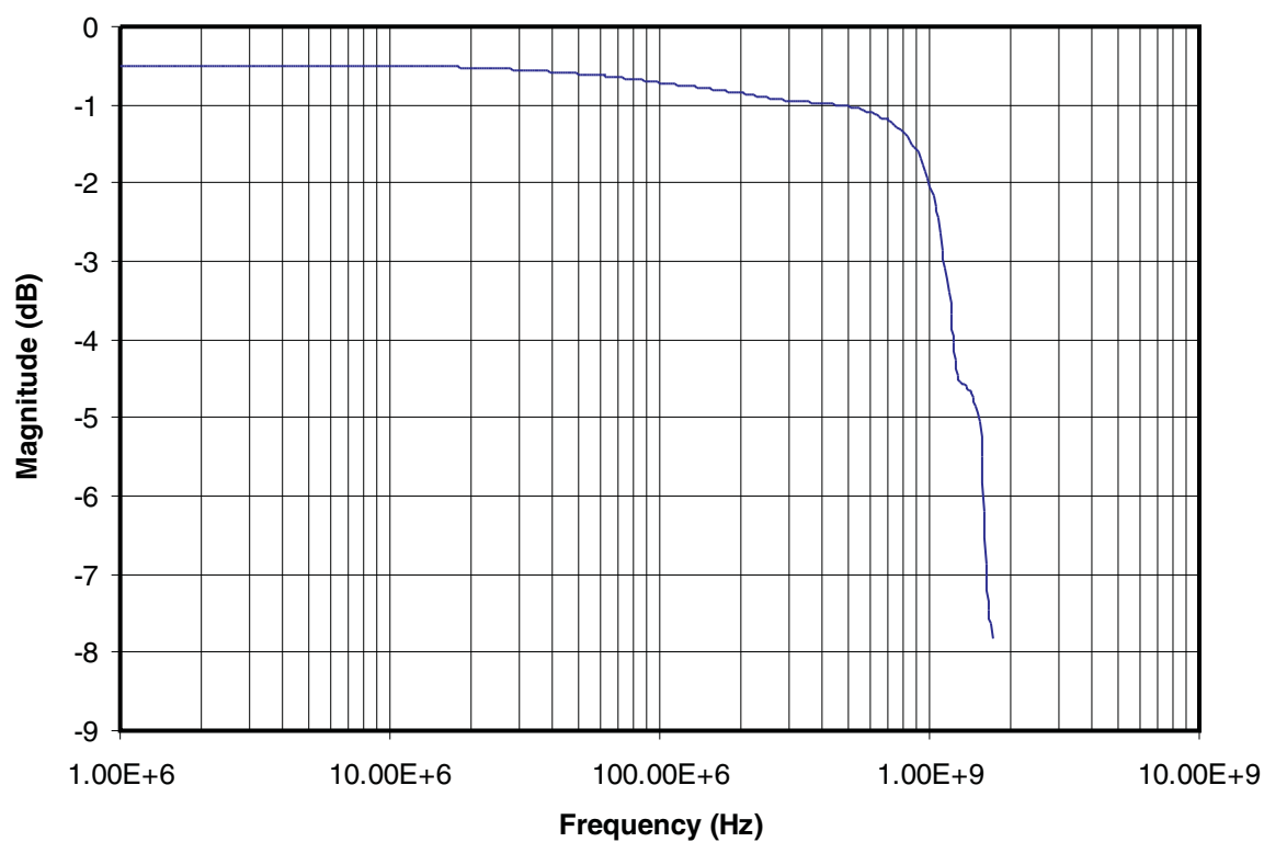
Figure 1. Insertion Loss
