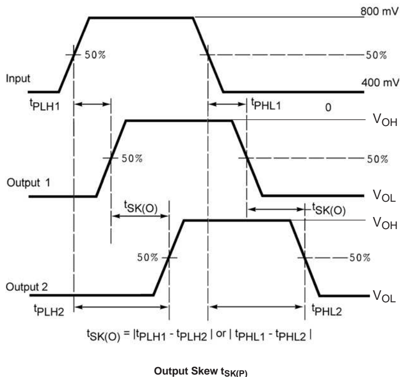
Figure 12. Skew Test
