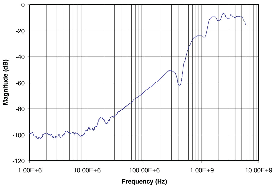
Figure 3. Crosstalk
