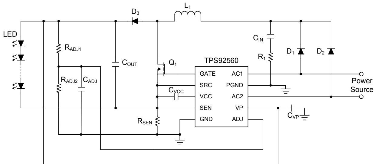
Typical application circuit of the TPS92560 using boost configuration
