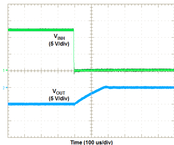
Figure 43. Inhibit Turn-Off
