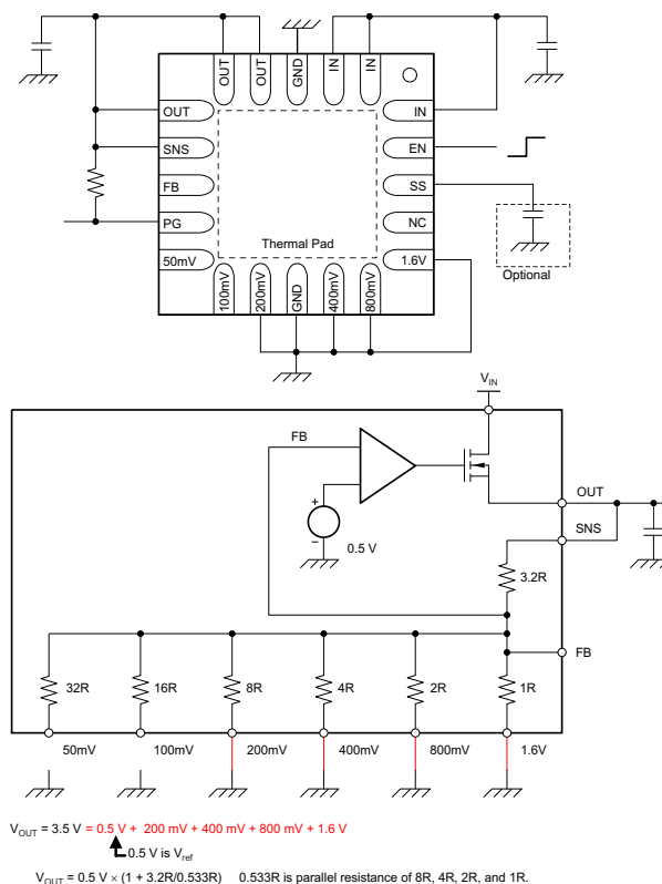
Figure 39. 3.5-V Configuration
