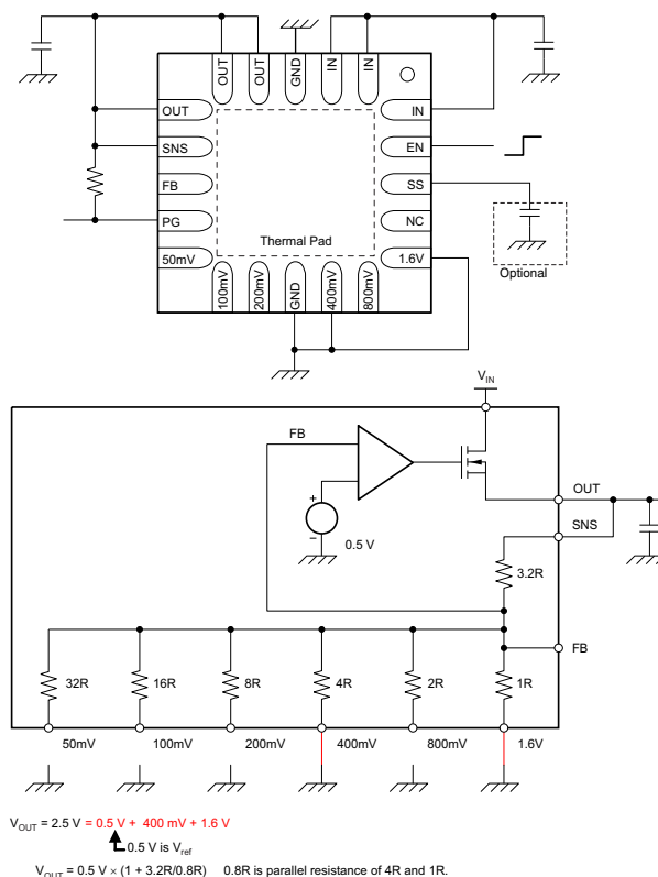
Figure 37. 2.5-V Configuration
