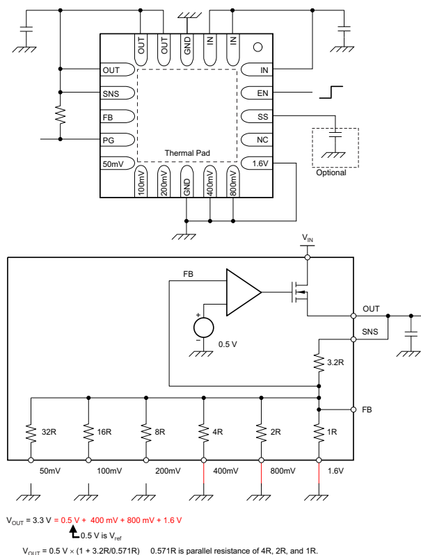
Figure 38. 3.3-V Configuration
