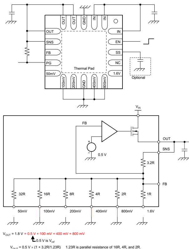
Figure 36. 1.8-V Configuration
