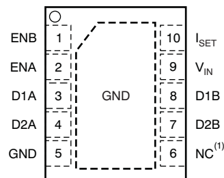
DSK PACKAGE 2,5mm × 2,5mm SON-10 (TOP VIEW)
