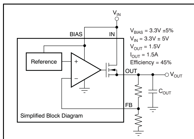
Figure 27. Typical Application of the TPS74801-Q1 Without an Auxiliary Bias Rail
