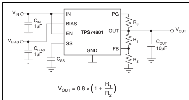
Figure 25. Typical Application Circuit for the TPS74801-Q1 (Adjustable)
