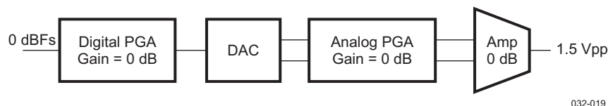
Figure 6-6. Headset Amplifier
