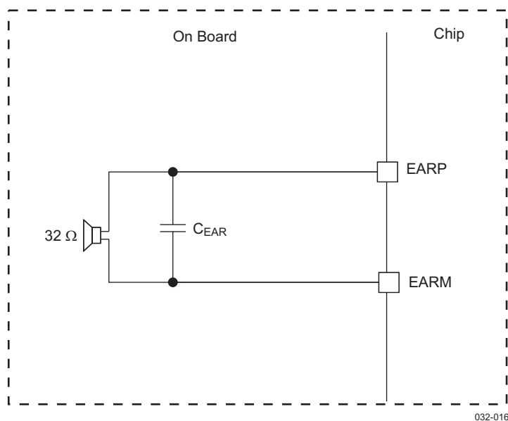
Figure 6-3. Earphone Speaker
