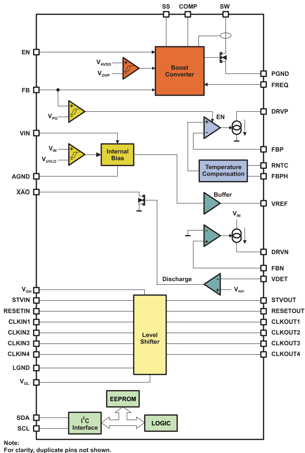
Figure 28. Internal Block Diagram
