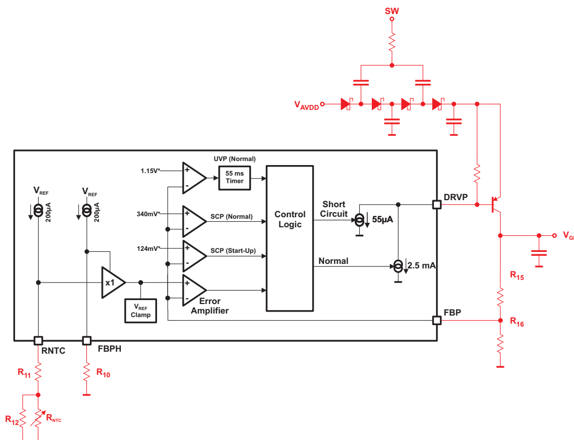
Figure 30. Positive Charge Pump Internal Block Diagram
