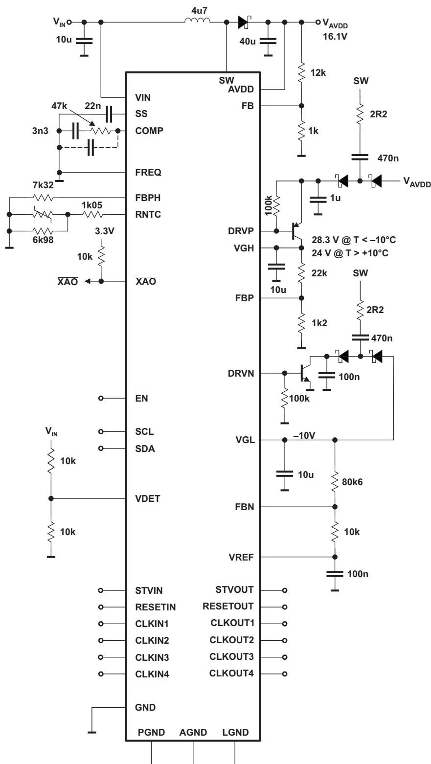
Figure 39. Typical Application Circuit Using Positive Charge Pump in ×2 Configuration
