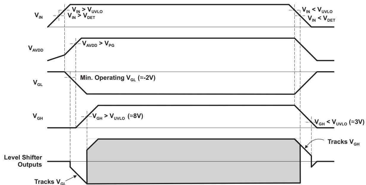
Figure 37. Power Supply Sequencing with EN Pin Tied to V_{IN} , V_{DET} < V_{UVLO}
