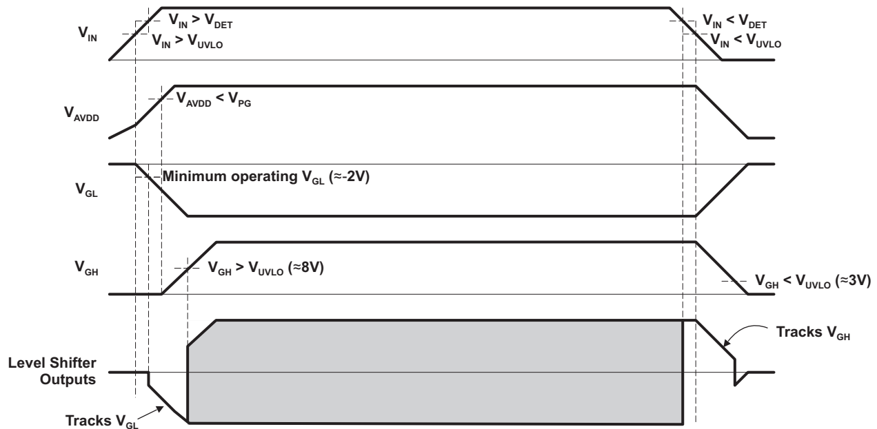
Figure 38. Power Supply Sequencing with EN Pin Tied to VIN, V_{DET} > V_{UVLO}
