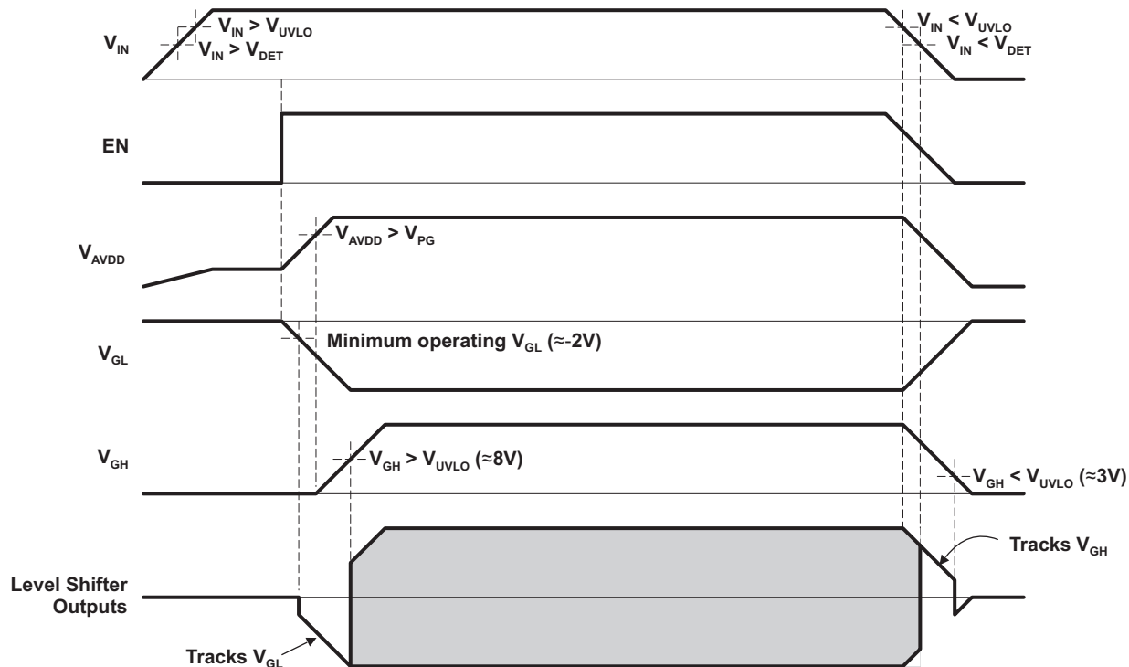
Figure 35. Power Supply Sequencing Using EN Pin, V_{\text{DET}} < V_{\text{UVLO}}
