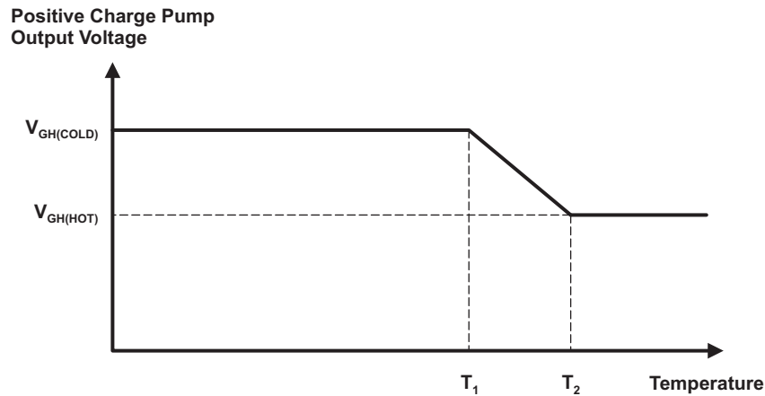
Figure 31. Positive Charge Pump Temperature Compensation
