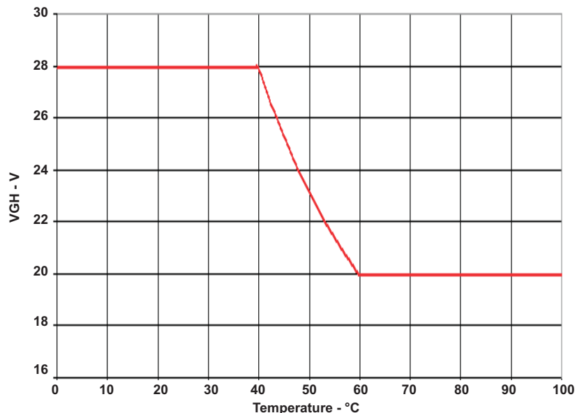
Figure 32. Temperature Compensated V GH
