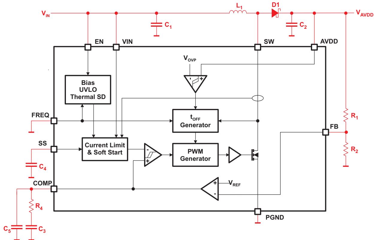
Figure 29. Boost Converter Internal Block Diagram
