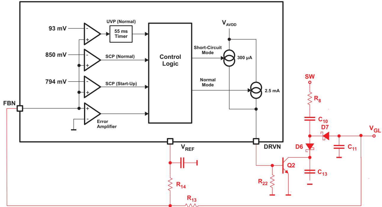
Figure 33. Negative Charge Pump Internal Block Diagram
