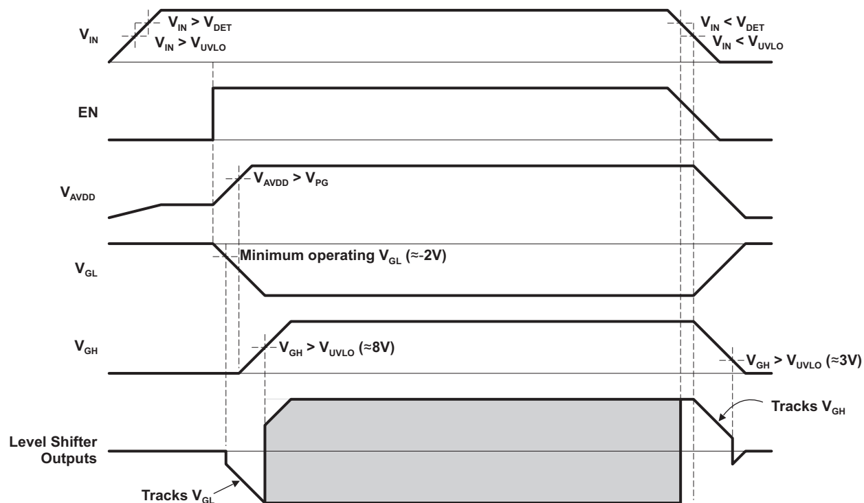
Figure 36. Power Supply Sequencing Using EN Pin, V_{DET} > V_{UVLO}
