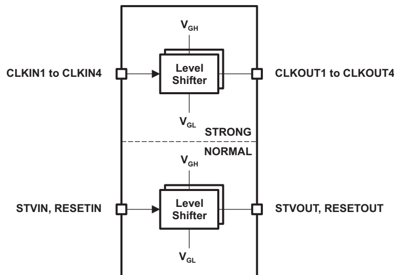
Figure 34. Level Shifter Block Diagram
