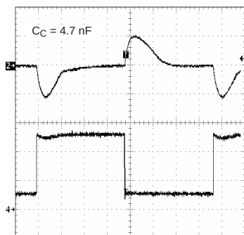
Figure 18. C_c = 4.7 nF
