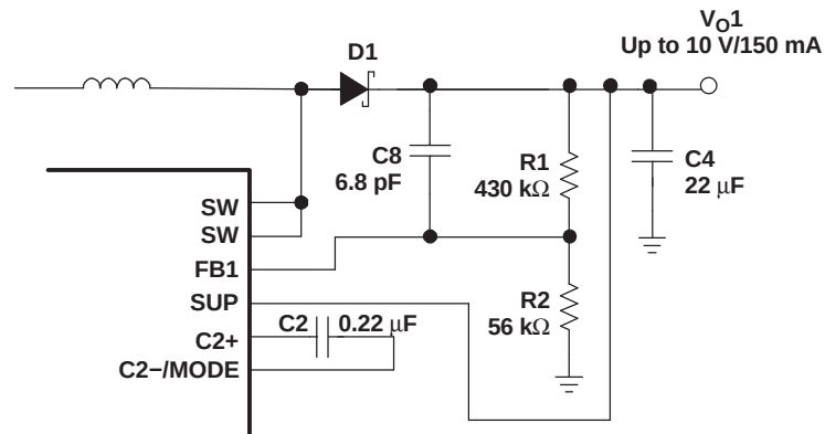
Figure 15. Feedforward Capacitor
