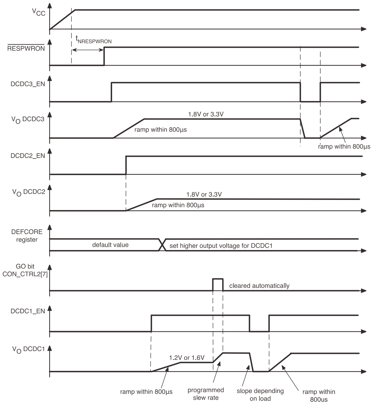
Figure 29. DVS Timing
