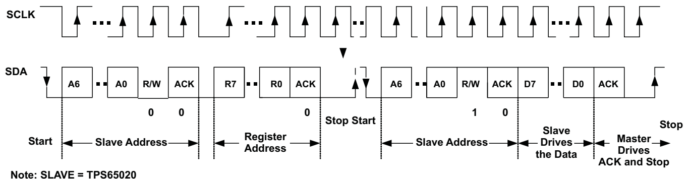
Figure 33. Serial i/f READ from TPS65022: Protocol B
