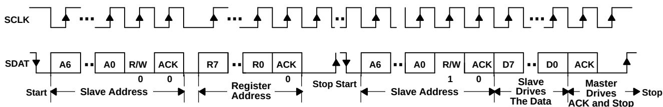
Figure 43. Serial Interface READ From TPS65014: Protocol B
