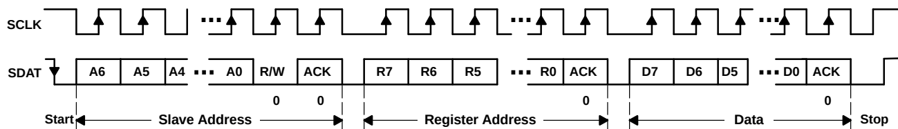
Figure 41. Serial Interface WRITE to TPS65014 Device
