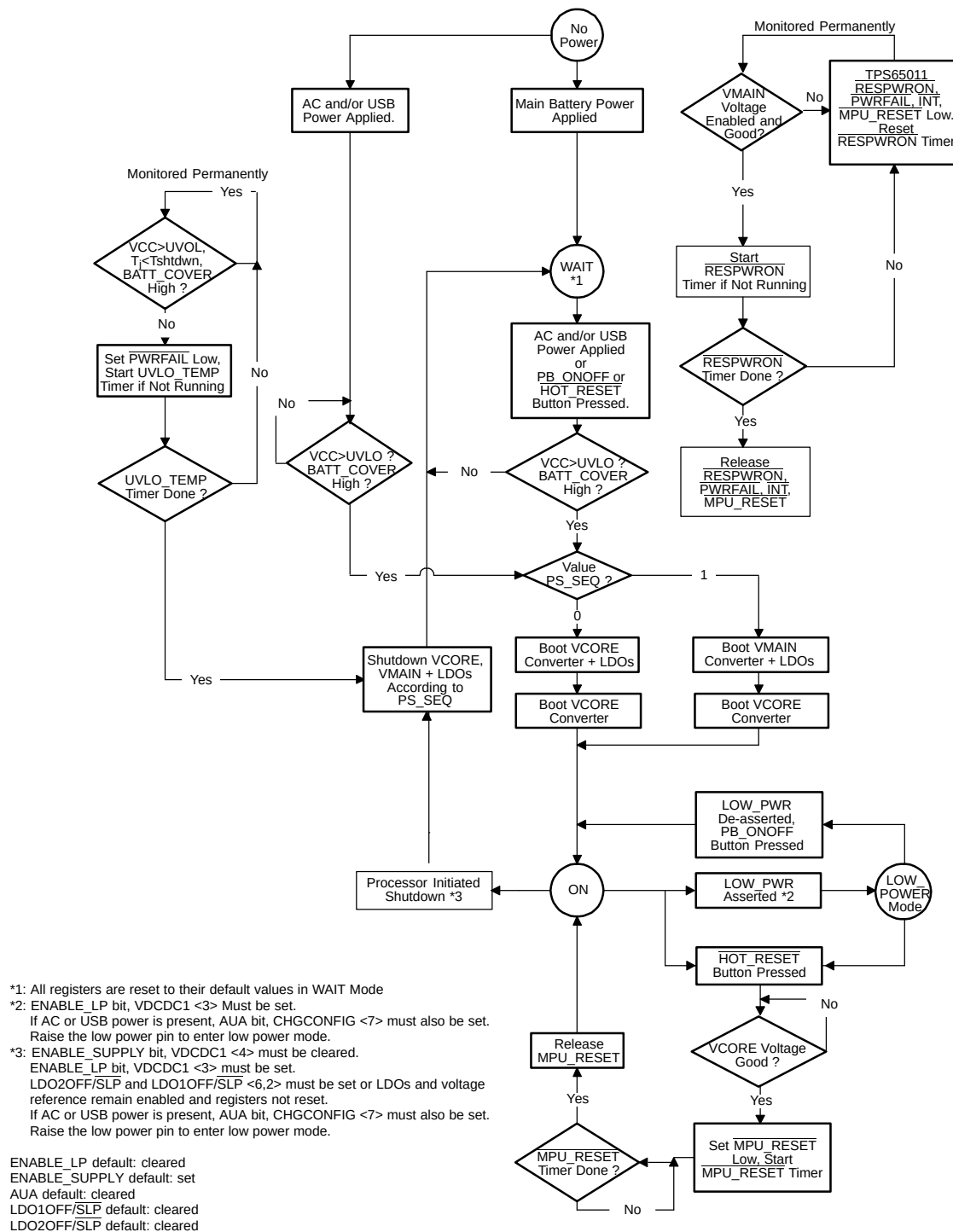
Figure 31. TPS65014 Power-On State Diagram
