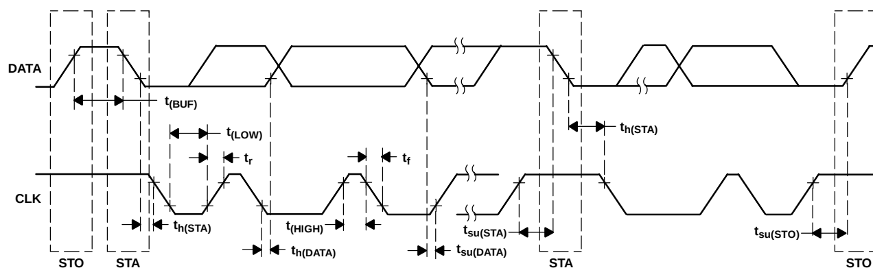
Figure 44. Serial Interface Timing Diagram
