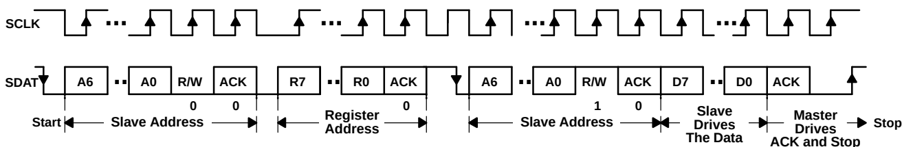
Figure 42. Serial Interface READ From TPS65014: Protocol A
