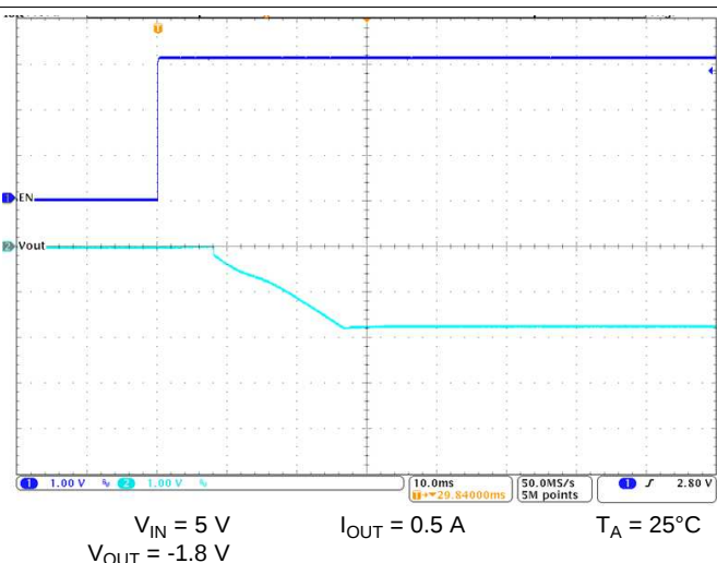
Figure 28. Start-Up Timing
