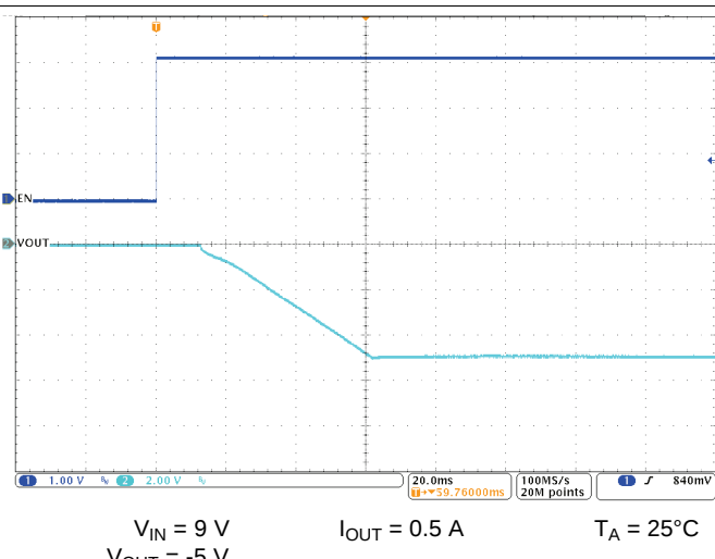
Figure 30. Start-Up Timing
