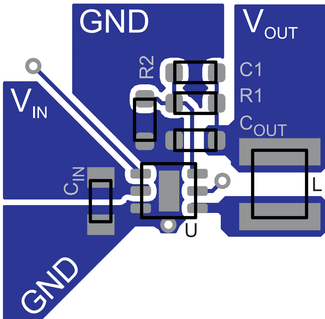
Figure 33. Suggested Layout for Adjustable-Output-Voltage Version
