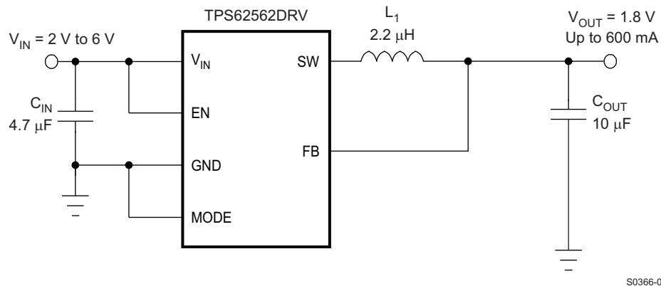
Figure 31. TPS62562 Fixed 1.8-V Output
