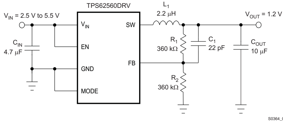
Figure 29. TPS62560 Adjustable 1.2-V Output
