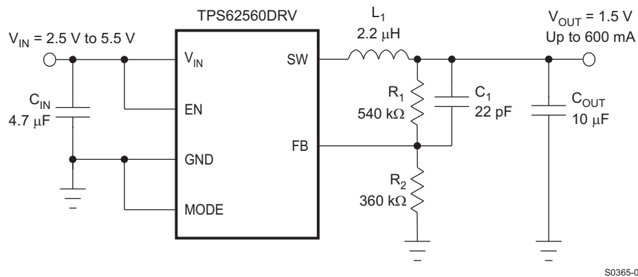
Figure 30. TPS62560 Adjustable 1.5-V Output
