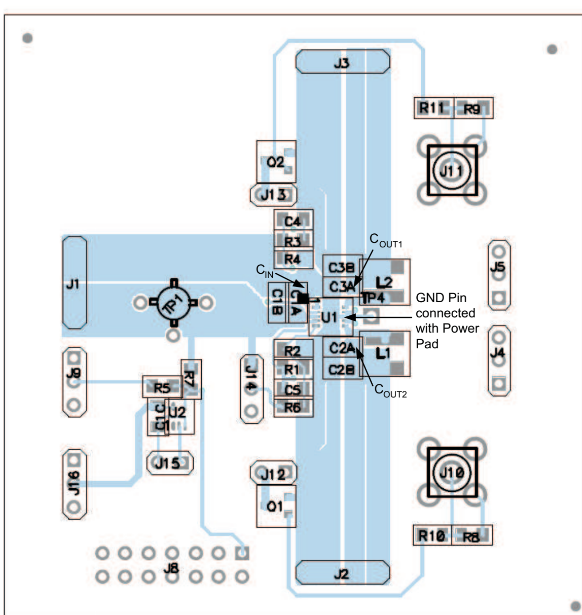
Figure 49. PCB Layout
