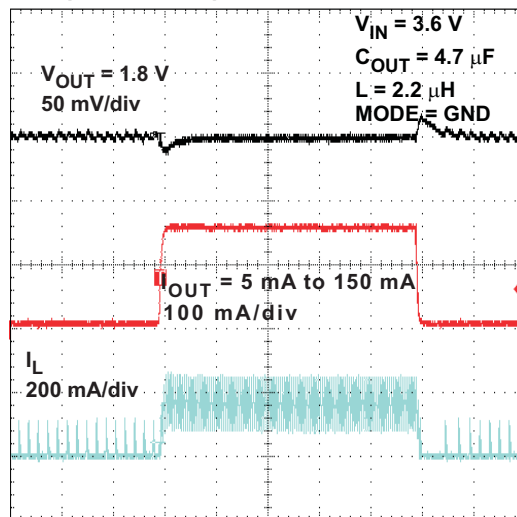
t - Time - 10 μs/div
