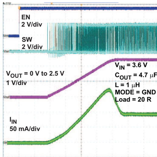
t - Time - 20 μs/div
