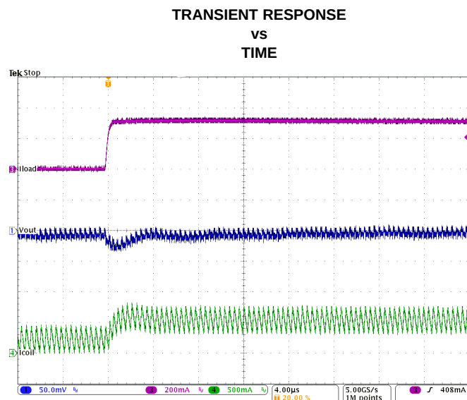
Figure 27. Load Transient Response in PWM Mode (200mA to 500mA), rising edge
