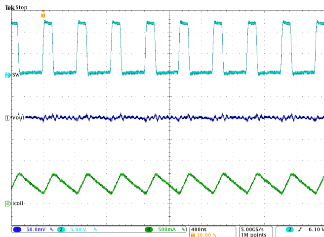
Figure 32. Typical Operation in PWM mode (I out =500mA)
