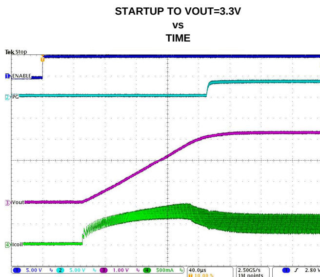
Figure 30. Startup with Iout=500mA
