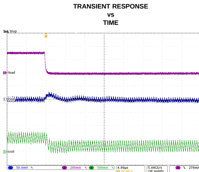
Figure 28. Load Transient Response in PWM Mode (200mA to 500mA), falling edge
