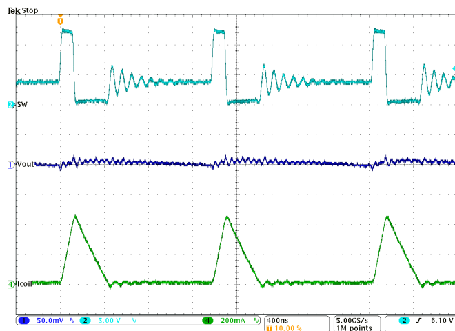
Figure 31. Typical Operation in Power Save Mode (I out =66mA)
