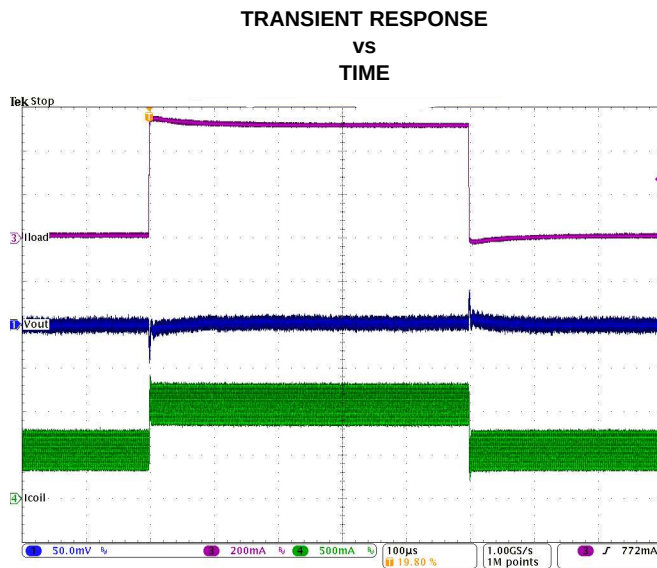
Figure 25. Load Transient Response in PWM mode (500mA to 1A)
