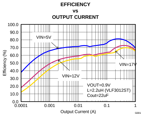
Figure 11. V_{out}=0.9V
