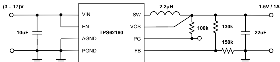
Figure 38. 1.5V/1A Power Supply
