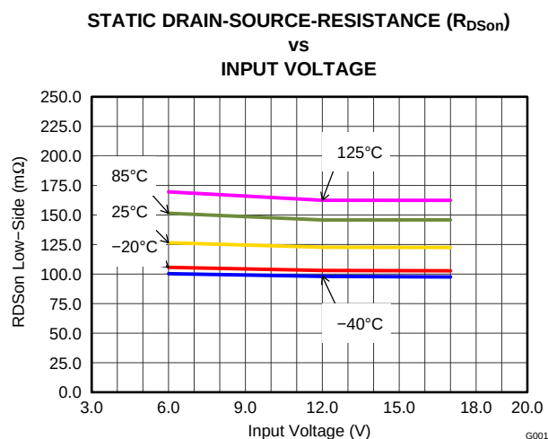
Figure 20. Low-Side Switch
