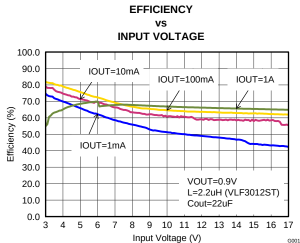
Figure 12. V_{out}=0.9V
