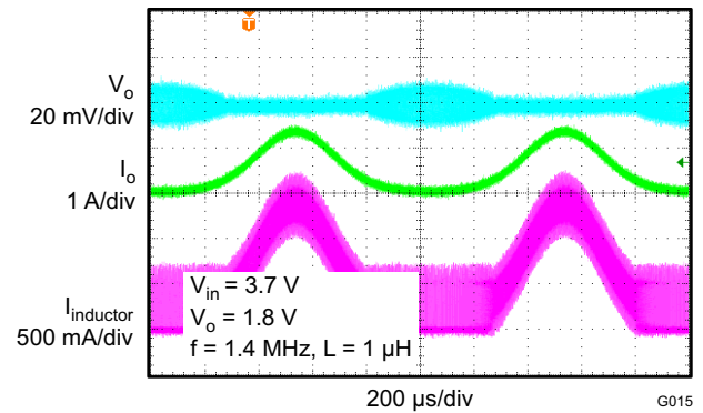
Figure 19. Load Sweep
