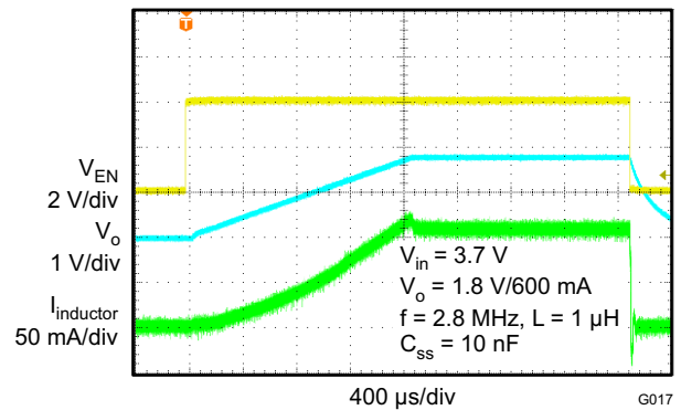
Figure 21. Start-Up
