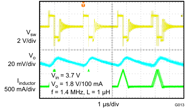
Figure 17. PFM Operation
