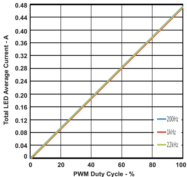
Figure 4. Dimming Linearity
