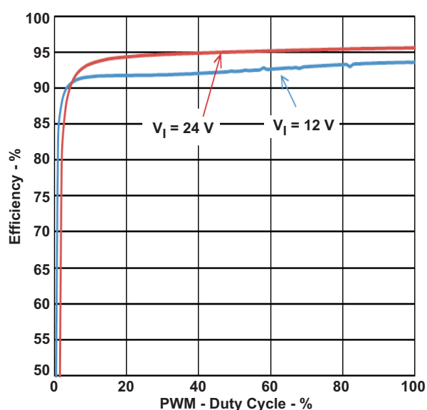
Figure 3. Dimming Efficiency
