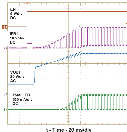
Figure 9. Startup Waveform
