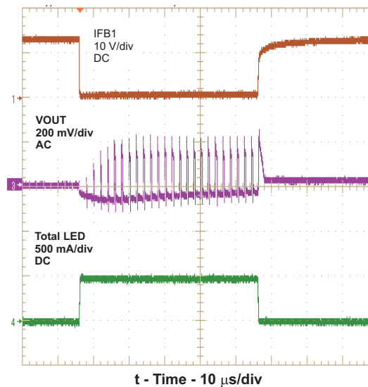
Figure 7. Dimming Waveforms
