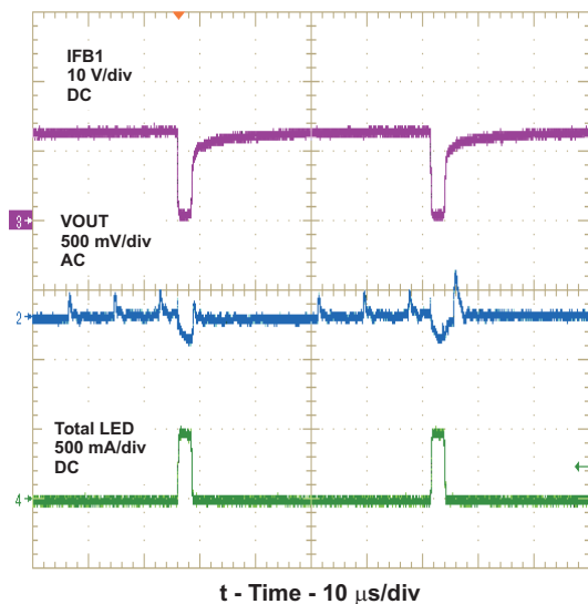
Figure 8. Dimming Waveforms
