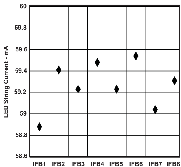
Figure 6. Current Matching
