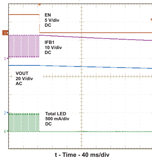
Figure 10. Shutdown Waveform
