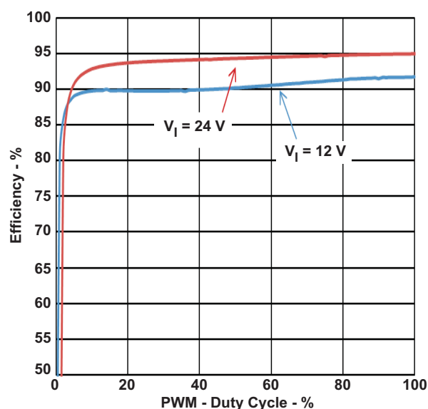
Figure 2. Dimming Efficiency
