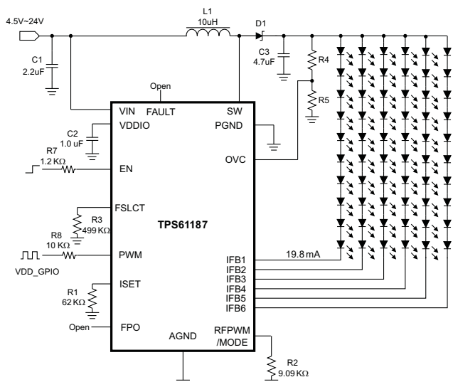
Figure 1. Typical Application – Phase Shift PWM Mode
