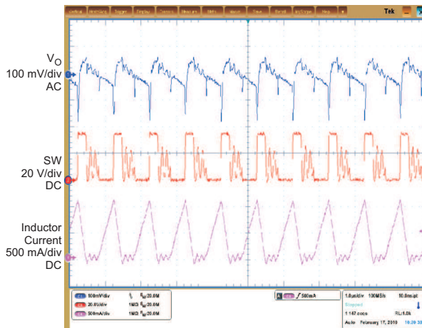
Figure 10. Switch Waveform
