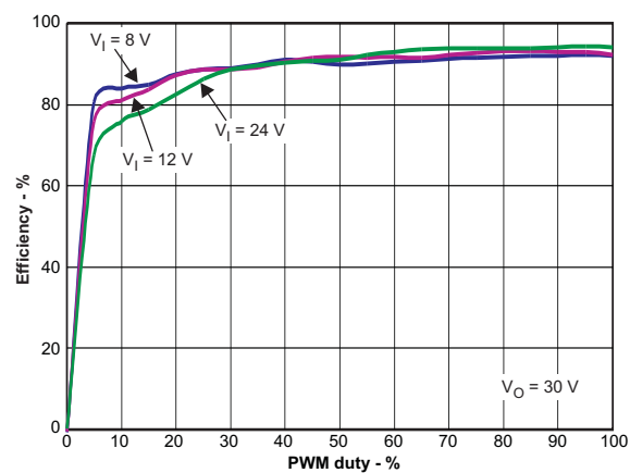
Figure 4. Efficiency
