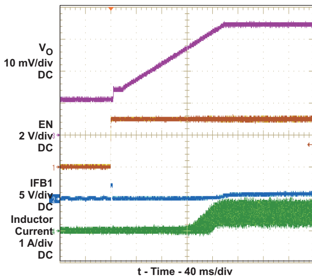
Figure 13. Startup Waveform
