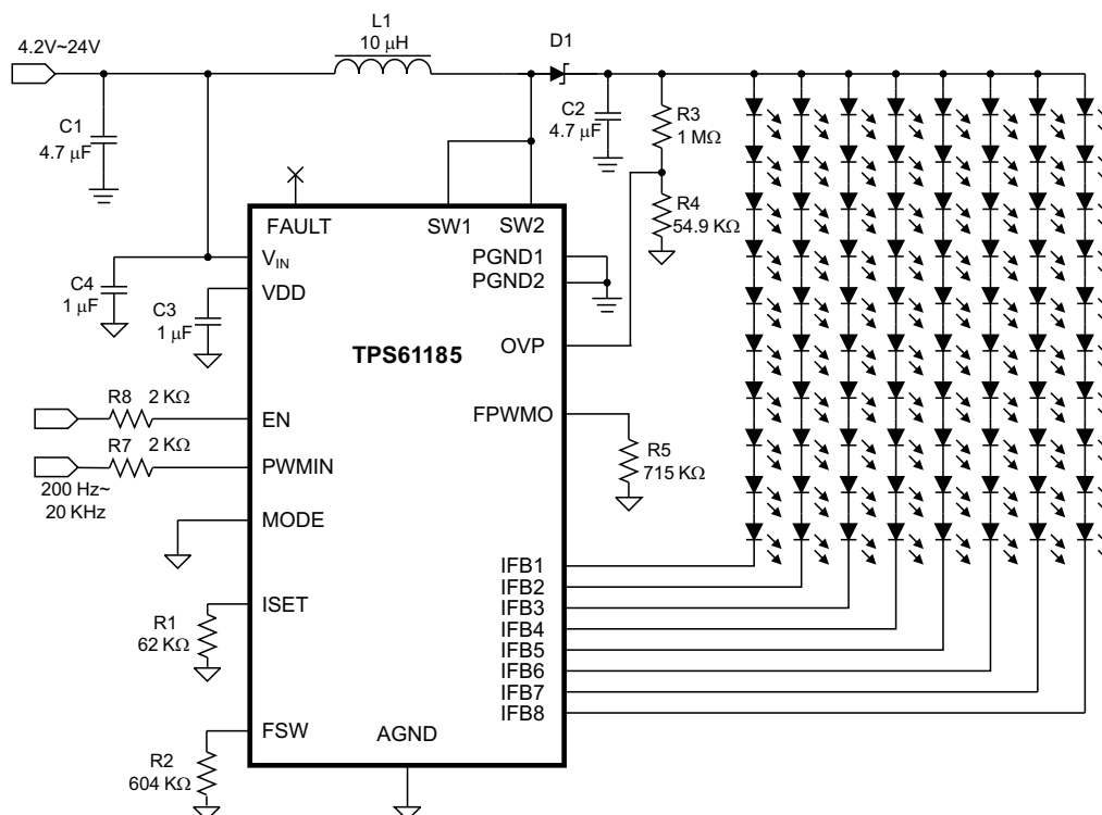
Figure 20. Typical Application Circuit for Direct PWM Dimming
