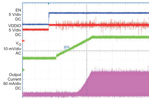
Figure 15. Start Up Waveform
