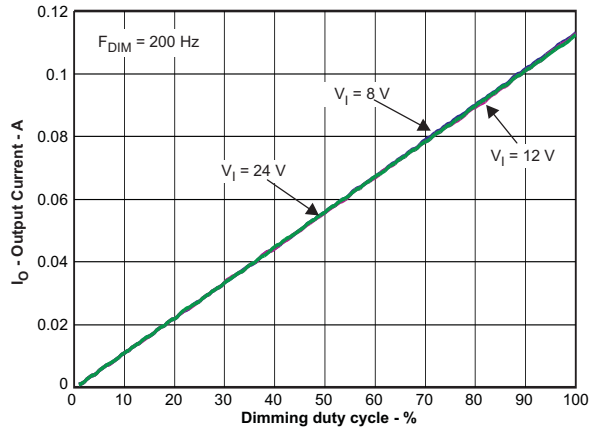
Figure 5. Dimming Linearity
