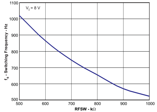
Figure 6. Boost Switching
