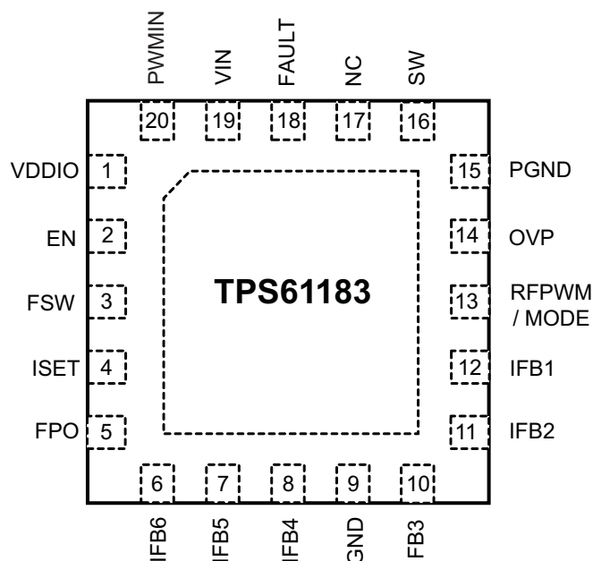
20 PIN 4mm × 4mm RTJ PACKAGE TOP VIEW
