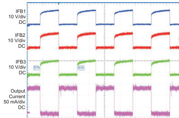
Figure 11. Programmable PWM Waveform
