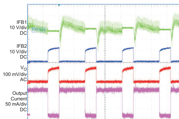
Figure 13. Output Ripple Waveform
