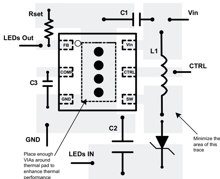
Figure 16. Sample Layout
