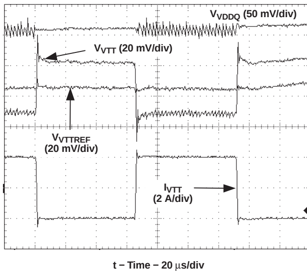
Figure 28. VTT Load Transient Response
