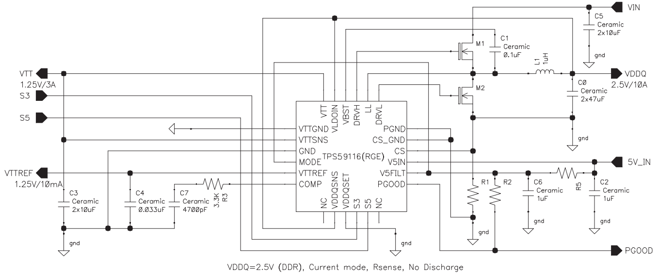
Figure 5. Current Mode
