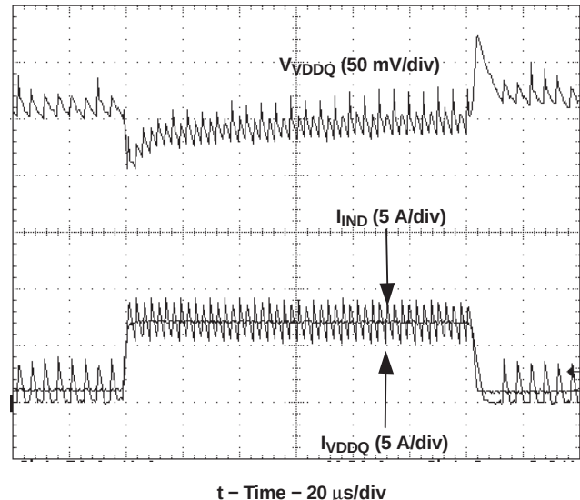
Figure 27. VDDQ Load Transient Response
