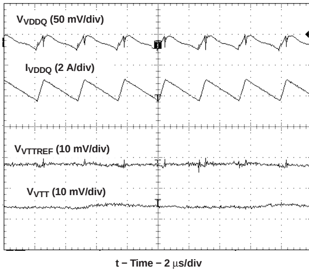
Figure 26. Ripple Waveforms - Heavy Load Condition
