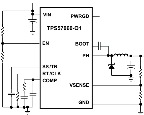
SIMPLIFIED SCHEMATIC
