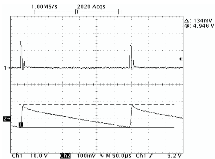
Figure 10. Low-Power-Mode Operation, I_L = 15 mA, C_O = 47 μF
