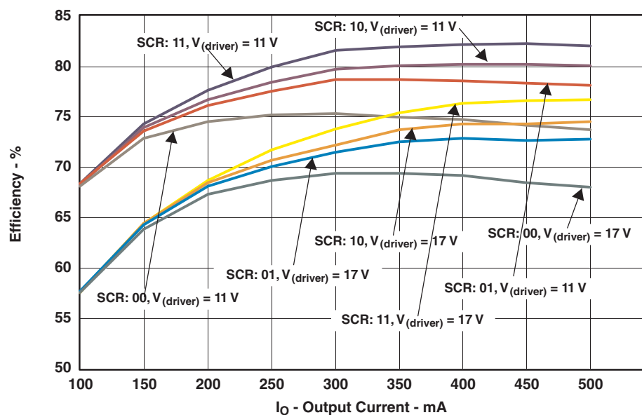
Figure 5. Converter Efficiency
