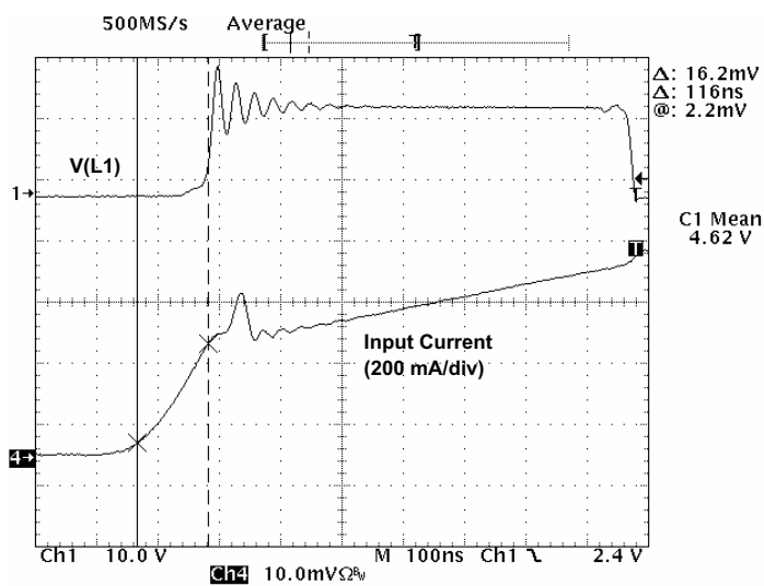
Figure 6. Input Current With Slope Control, SCR0 = 0, SCR1 = 0, Input-Current Slew Rate = 2.8 \text{ A}/\mu\text{s} , I_L = 500 \text{ mA} , V_{(driver)} = 15 \text{ V}
