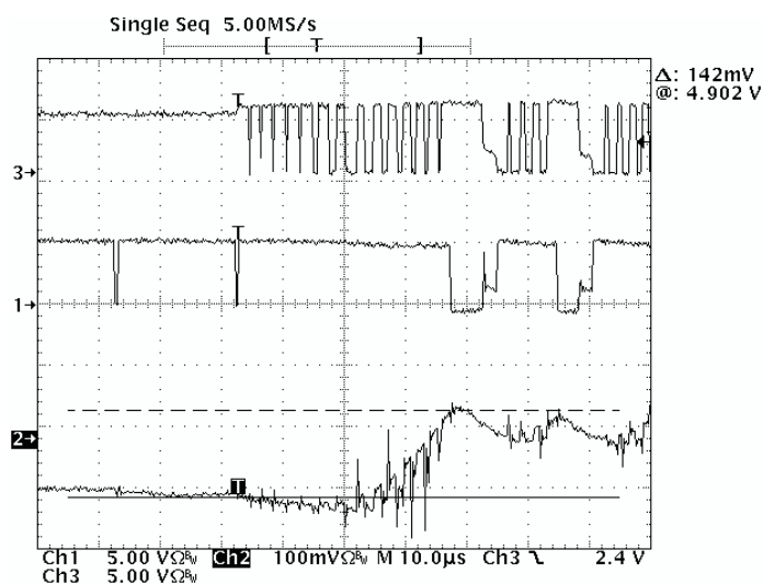
Figure 16. Switch-Mode Regulator Transition From Buck Mode to Boost Mode, I_L = 400 mA
