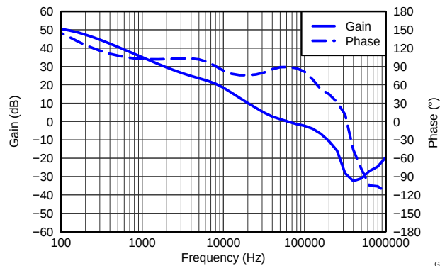
CLOSED LOOP RESPONSE, I_{OUT} = 4 A
