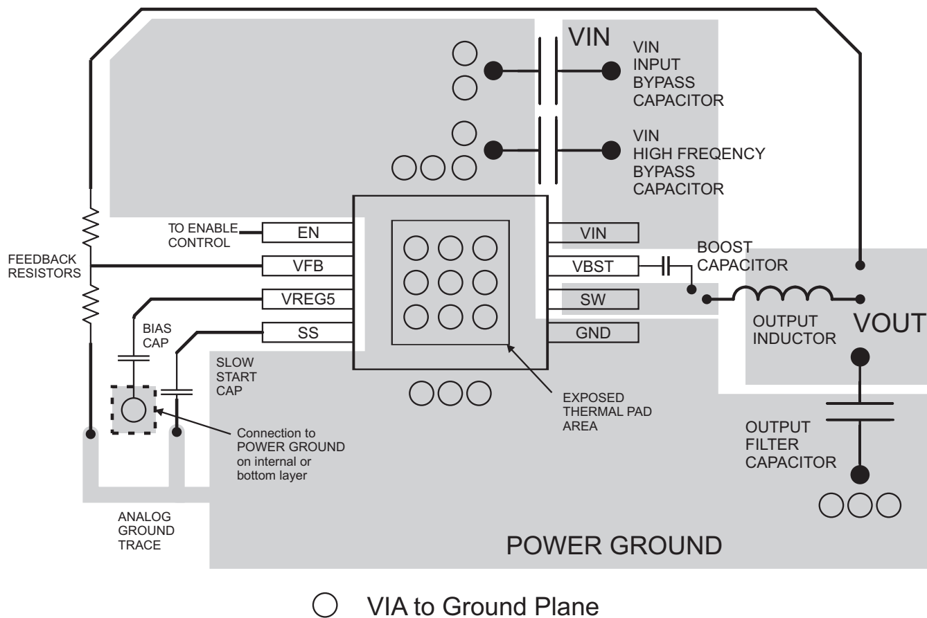
Figure 18. PCB Layout
